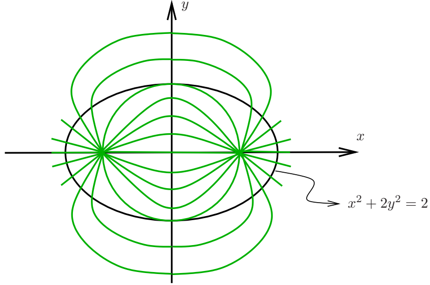
FIGURE 5. The intersection of the “pages” of (\tilde{K}, \tilde{\theta}) with the xy -plane, and the ellipse x^2 + 2y^2 = 2 .
