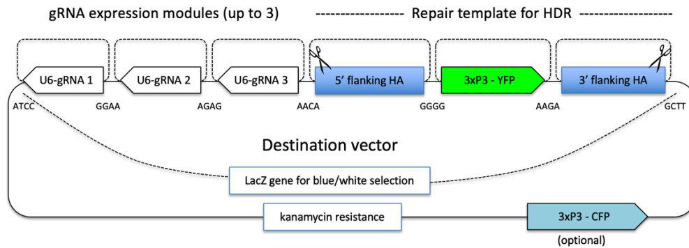
Figure 1: Plasmid map of the gRNA expression and repair template vector for injection into Cas9-expressing mosquito embryos. Inserts (gRNA expression modules, regions of homology, fluorescence marker) are assembled from ampicillin-resistant plasmid modules or PCR products in the destination vector by Golden Gate Cloning (GGC) using BsaI sites whose variable 4-base overhangs are indicated (top strand nucleotides). The single-tube restriction-ligation GGC reaction removes a LacZ cassette allowing blue-white screening, resulting in white positive colonies. Ampicillin-resistant backbones that are lost upon the GGC reaction are represented as dashed lines. The number of gRNAs may be reduced to 2 by short-circuiting the assembly with module pKSB- gRNA 2/3 (Addgene #173674), or to 1 by short-circuiting the assembly with a short linker. HA = homology arms to promote homologous recombination-mediated repair of the genomic Cas9 break. Scissors show the position of gRNA target sites that can be incorporated at the extremities of the HAs to promote plasmid linearization by Cas9 upon injection. U6-gRNA1, 2, 3 plasmids are available from Addgene (#173671—3) as well as destination vectors (#173668; 62289—95). A fluorescence marker in the backbone of the vector, different from the marker in the repair template, can help identify non-canonical integration events that integrate the entire plasmid in the mosquito genome.
