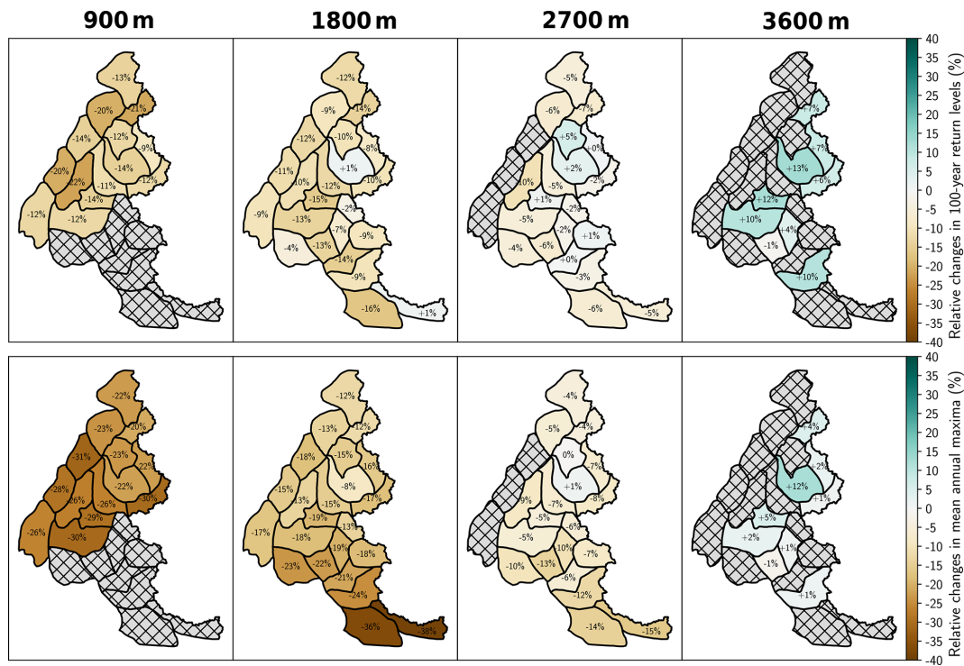
Figure 2. Relative changes in mean annual maxima and 100-year return levels of daily snowfall between the current climate (corresponding here to +1 °C of global warming) and +4 °C of global warming at elevations 900, 1800, 2700, and 3600 m. Hatched gray massifs denote massifs that are not available (Sect. 3, second step of our analysis).
