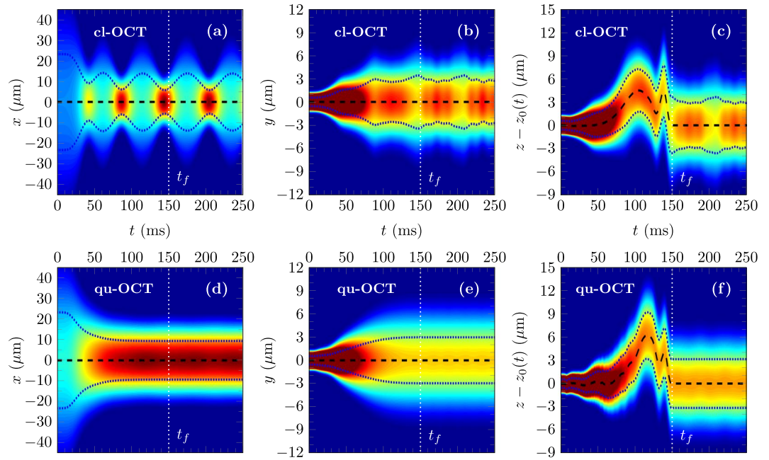
Figure 3. Condensate dynamics in the x , y and z directions using the cl-OCT ramp (upper line) and the qu-OCT ramp (lower line) shown in Fig. 2. The transport duration is t_f=150 ms. The average atomic density, solution of the time-dependent Gross-Pitaevskii equation, is shown as a function of time and position: (a) and (d) P_x(x, t) , (b) and (e) P_y(y, t) , (c) and (f) P_z(z, t) . The black dashed lines show the expected center of mass trajectory. The dotted blue lines highlight the expected width dynamics according to the scaling approach. The dotted vertical white lines mark the time of the end of the transport. The total atom number is N=10^5 . See text for details.
