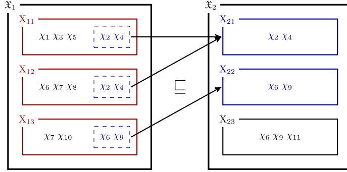
Fig. 1. Two hypertteams with \mathfrak{X}_1 \sqsubseteq \mathfrak{X}_2 , but \mathfrak{X}_2 \not\sqsubseteq \mathfrak{X}_1 .
