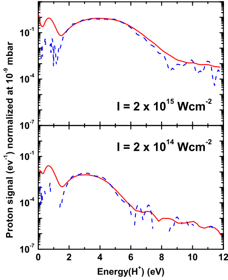
FIG. 4. (Color online) Proton spectra from \text{H}_2 recorded with linearly polarized 40 fs laser pulse at I=2 \times 10^{14} and 2 \times 10^{15} \text{ W cm}^{-2} . For each laser intensity, the full curve represents the total proton spectrum and the dashed curve represents the covariance proton spectrum from the \text{H}^+ + \text{H}^+ dissociation channel.
