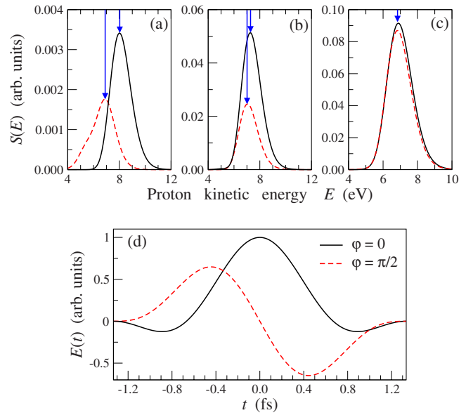
FIG. 13. (Color online) Calculated proton spectra from H_2 at 8 \times 10^{14} \text{ W cm}^{-2} as a function of the carrier-envelope phase \varphi and the pulse duration. Full curves: \varphi = 0 . Dashed curves: \varphi = \pi/2 . The left (a), middle (b), and right (c) top panels correspond to different pulse durations of, respectively, 1, 2, and 4 fs. The vertical arrows mark the positions of the different peaks. The corresponding electric field is represented in the bottom panel (d) as a function of time for a pulse duration of 1 fs.
