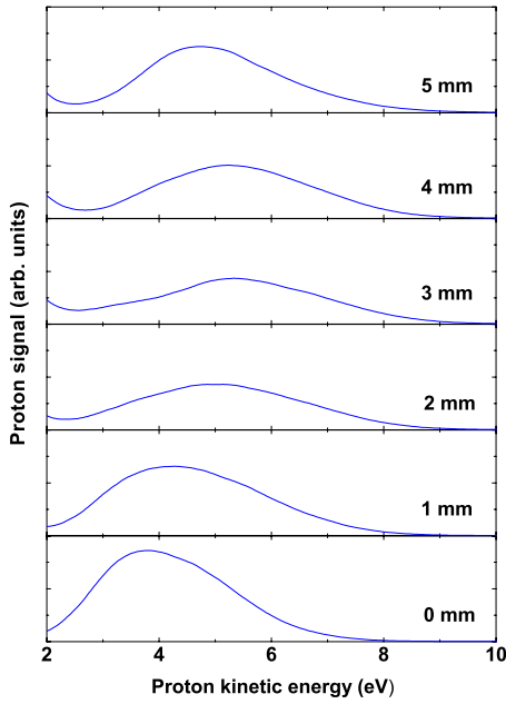
FIG. 12. (Color online) Optimization of the ultrashort pulse duration. Proton spectra from H_2 recorded at 2 \times 10^{15} \text{ W cm}^{-2} with different thicknesses of fused silica from 0 to 5 mm inserted in the beam path before the ion spectrometer.
