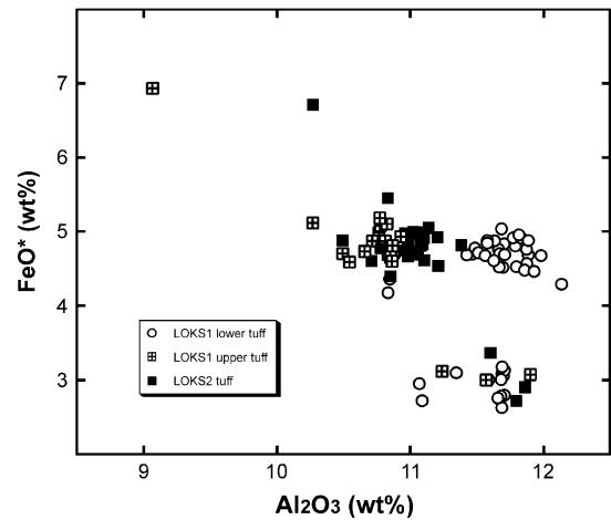
Fig. 2. FeO total versus Al 2 O 3 for glass shards contained in LOKS1 and LOKS2 tuffs. The concentrations have been recalculated to 100% on an H 2 O-free basis.
