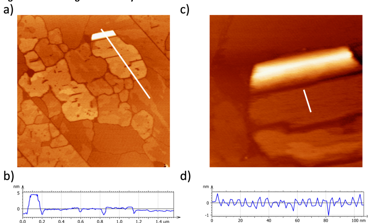
a) Large-scale ( 2 \times 2 \mu\text{m}^2 ) topography AFM of multilayers of EsterOC18 molecules deposited on a HOPG surface. b) Z-profile taken along the white line of showing the formation of islands with different apparent height. c) Zoom ( 600 \times 600 \text{ nm}^2 ) over multilayered islands are constituted of bright lines separated by darker stripes. d) Z-profile taken along the white line of c).
