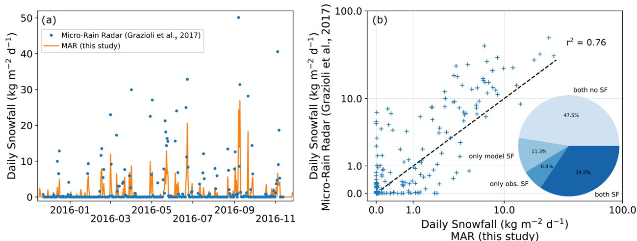
Figure A4. Evaluation of the ability of MAR to match the snowfall timing observed with micro-rain radar at Dumont D’Urville station (66° S, 140° E; Grazioli et al., 2017). Micro-rain radar data indicate snow passing through the atmospheric layer 300 m above the surface, while the modelled snowfall is shown for the surface only, where some of the snow may have sublimated. (a) Time series of modelled and observed snowfall for the year 2016. (b) Scatterplot of observed vs. modelled snowfall. The pie chart indicates the percentage of days with matching or mismatching snowfall in the model and observations, with discrepancies noted for about 18 % of the days in total.
