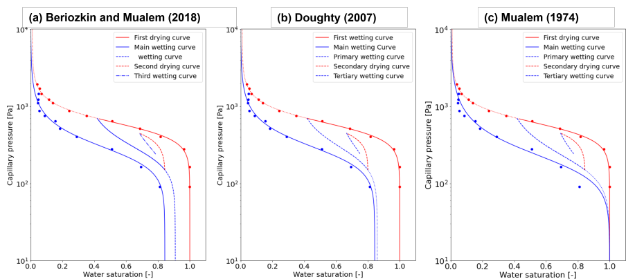
Figure 14: Illustration of the hysteresis effect on retention curve properties of Sand 40/50. Scanning loops are calculated with different models. (a) Beriozkin, Mualem (2018) . (b) Doughty (2007) . (c) Mualem (1974) .
