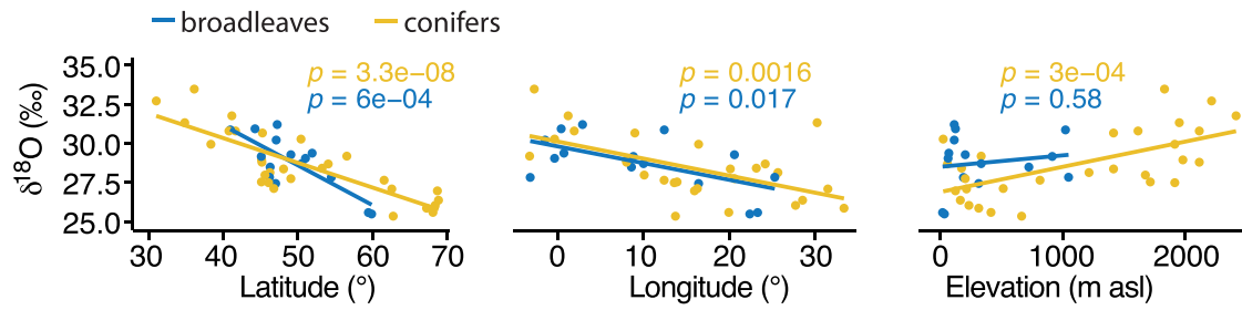
Extended Data Fig. 1 | Dependency of mean \delta^{18}\text{O} site values of the common period 1900-1994 on geographic location. p-values below 0.05 indicate significant relationships.
