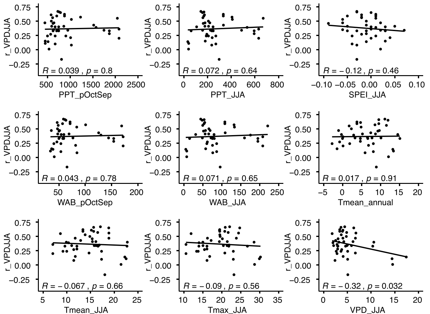
Extended Data Fig. 4 | Relationship between climate- \delta^{18}\text{O} correlations and long-term means (period 1920-1994) of precipitation sums (PPT), SPEI, water balance (WAB), mean temperature ( T_{\text{mean}} ), maximum temperature ( T_{\text{max}} ) and VPD. Each point indicates a correlation coefficient calculated between a site \delta^{18}\text{O} chronology and the closest gridpoint climate dataset,
