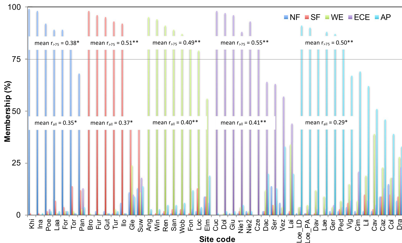
Extended Data Fig. 5 | Contribution of the individual site chronologies to the common variance in the regional clusters of Northern Fennoscandia (NF), Southern Fennoscandia (SF), Western Europe (WE), Eastern Central Europe (ECE) and Alps & Pyrenees (AP). Membership (%) the contribution to the common variance in a cluster in percentage. Mean r_{all} is the mean inter-series correlation coefficient (that is, the common signal strength) of all chronologies
