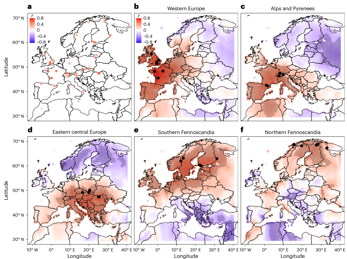
Fig. 2 | Spatial extend of the summer VPD signal in five European target regions. a ) Correlation between individual site \delta^{18}\text{O} chronologies and the closest summer VPD gridpoint. b–f ) Spatial correlation fields calculated between the PCI nests representing each of the five geographical regions derived from cluster analysis and gridded summer VPD (June–August). Large black dots indicate sites
