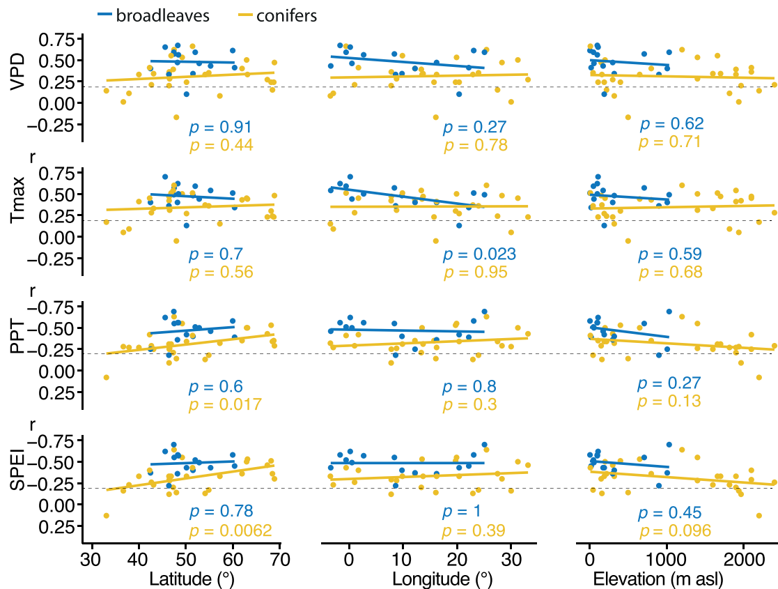
Extended Data Fig. 3 | Relationship between climate- \delta^{18}\text{O} correlations and geographic location for VPD, T_{max} , precipitation (PPT) and SPEI in summer (June to August). Each point indicates a correlation coefficient calculated between a site \delta^{18}\text{O} chronology and the closest gridpoint dataset, plotted as a function of latitude, longitude and elevation. Points above the dashed horizontal
