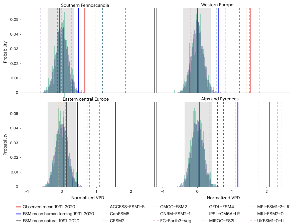
Fig. 4 | Unprecedented summer VPD increase in the context of pre-industrial natural variability and its attribution to human influence. Bars indicate pre-industrial natural variability from tree-ring \delta^{18}\text{O} -based VPD reconstructions for the period 1600-1850 (green), and from 500-year simulations of 12 ESMs with no human-induced forcing included, piControl (blue). Grey shadows represent the 98% distribution range of natural variability. Solid lines indicate VPD during the most recent period 1991-2020 CE based on i) direct VPD observations (red), ii)
