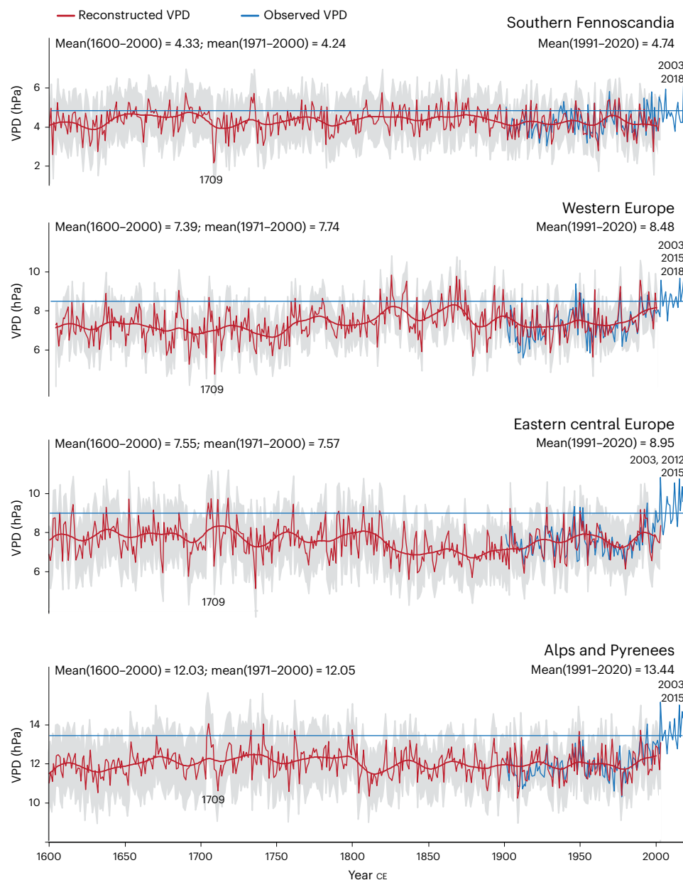
Fig. 3 | Reconstructed and observed summer (June–August) VPD for four European target regions. Horizontal blue lines indicate the mean of observed VPD for the period 1991–2020. Smoothed curves are 30-year splines with a frequency cut-off at 50%. Means and standard deviations (SD) are
