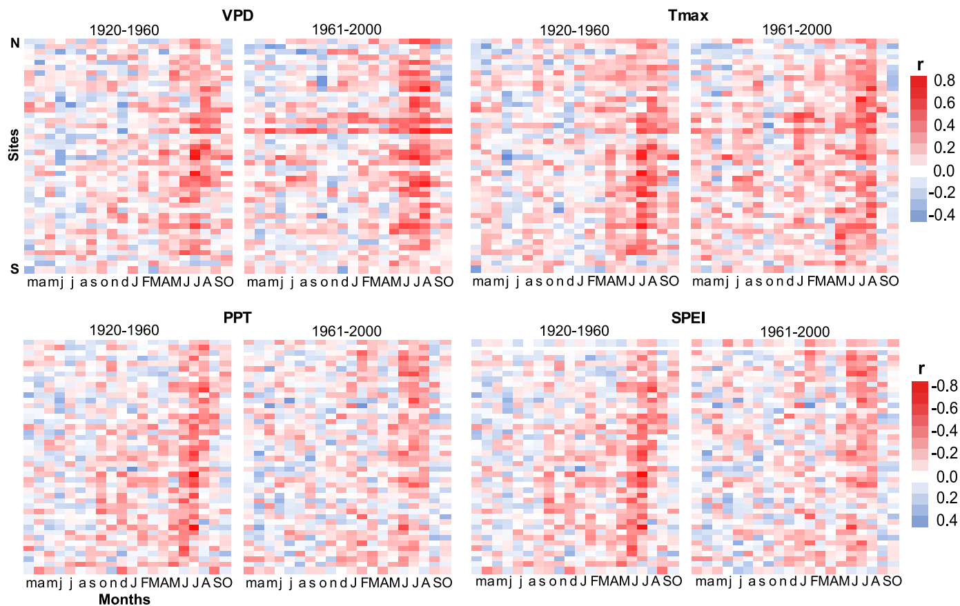
Extended Data Fig. 2 | Climate sensitivity of the site tree-ring \delta^{18}\text{O} chronologies in two independent time periods. Periods cover 1920-1960 and 1961-2000; shorter for those records that end in 1994, 1996 and 1998, (see Extended Data Table 1). Colours indicate Pearson's correlation coefficients calculated between each of the 45 site \delta^{18}\text{O} chronologies of the network and the
