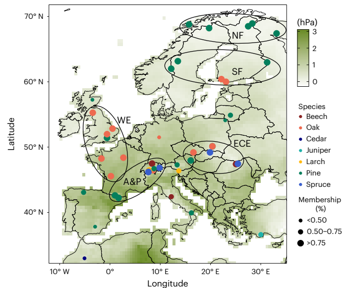
Fig. 1 | Distribution of 45 tree-ring cellulose \delta^{18}\text{O} chronologies across Europe, spatial clustering and changes in observed European summer VPD. Dot sizes indicate the contribution (membership in %) of the individual site chronologies to the common variance of a given cluster based on fuzzy cluster analysis (Extended Data Fig. 5). The chronologies are separated into five independent target regions, that is, northern Fennoscandia (NF), southern Fennoscandia (SF), western Europe (WE), eastern central Europe (ECE) and Alps & Pyrenees (AP). Green shadings represent differences in mean observational VPD between the period 1920–1990 and 1991–2020 calculated for each grid point based on the CRU TS 4.05 dataset. Map source: R package ggplot2 ( https://ggplot2.tidyverse.org ), R-version 4.1.2.
