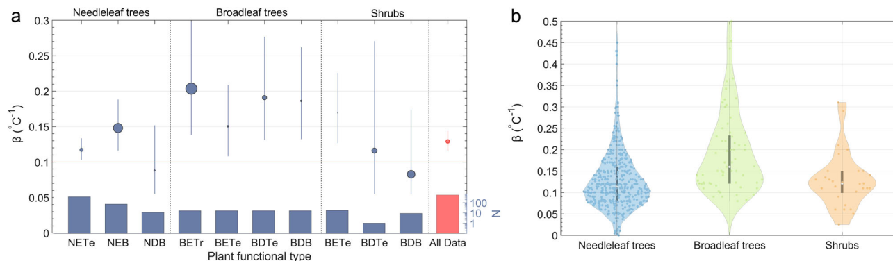
Fig. 4 Plant functional type-dependent \beta coefficients. Dependence on temperature ( \beta ) for the plant functional types (a) and wider categories of woody plants (b). The error bars in panel a indicate 95% confidence intervals, and the size of the blue bullet points is proportional to the global surface area of each plant functional type. NETe needleleaf evergreen temperate forest, NEB needleleaf evergreen boreal forest, NDB needleleaf deciduous boreal forest, BETr broadleaf evergreen tropical forest, BETe broadleaf evergreen temperate forest/shrubs, BDTe broadleaf deciduous temperate forest/shrubs, BDB broadleaf deciduous boreal forest/shrubs.
