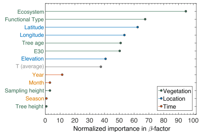
Fig. 3 Feature importance ranking. Indicative contribution of individual parameters of vegetation, location, and time parameters to the variation of the \beta coefficient. The parameters are explained in Supplementary Table 1.
