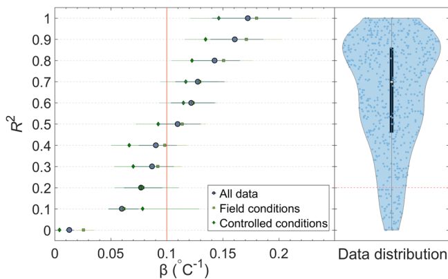
Fig. 2 Groups of coefficients of determination ( R^2 ) for experimentally derived dependencies ( \beta ) of MT emissions on temperature. The blue and green error bars indicate 95% confidence intervals. On the right, the distribution of the N = 696 values of \beta extracted from the literature is displayed together with a boxplot that illustrates their median (white circle) and 25th and 75th percentiles (lower and upper bounds of the box), respectively. Data below the red dashed line (on the right) were obtained from regressions with poor goodness of fit ( R^2 < 0.2 ) and were excluded from further analysis.
