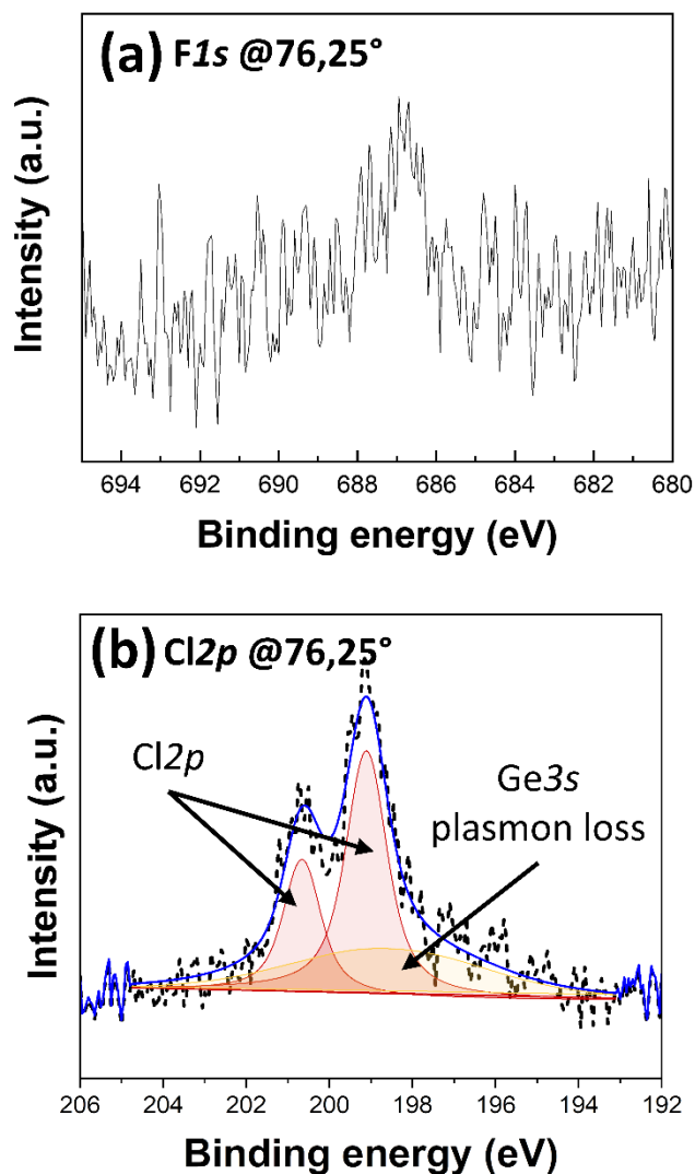
FIG. 3: (a) Typical F1s peaks at a collection angle of 76.25^\circ after HF immersion for 5 min and water rinse. (b) Typical Cl2p peaks at a collection angle of 76.25^\circ after HCl immersion for 5 min.
