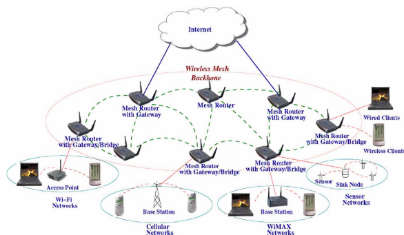
FIGURE 1. Wireless Mesh Network architecture [6].
