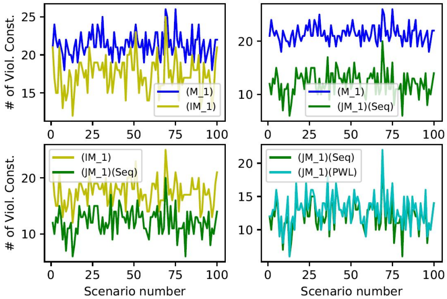
Fig. 3 Number of violated constraints for each randomly generated instance using K = 30 , \alpha = 0.25 and \sigma = 1
