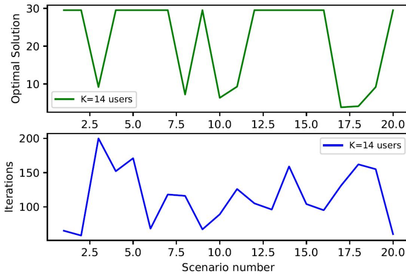
Fig. 6 Optimal solutions and the number of iterations obtained with Algorithm 2 for 20 initial samples of parameters \delta and \beta using K = 14 .
