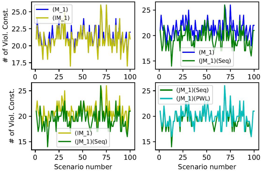
Fig. 1 Number of violated constraints for each randomly generated instance using K = 30 , \alpha = 0.25 and \sigma = 0.1
