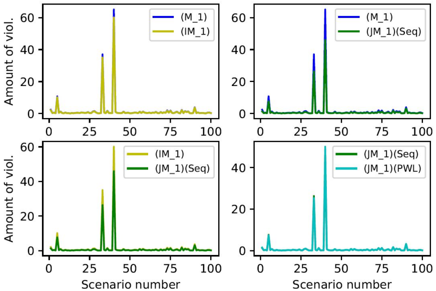
Fig. 2 The total amount of constraint violation for each randomly generated instance using K = 30 , \alpha = 0.25 and \sigma = 0.1
