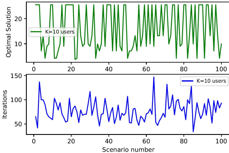
Fig. 5 Optimal solutions and the number of iterations obtained with Algorithm 2 for 100 initial samples of parameters \delta and \beta using K = 10 .
