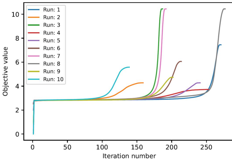
Fig. 7 Slow convergence of the condensed sequential approximation method reporting optimal solutions and the number of iterations obtained for an instance of K = 16 users while using different initial values of parameters \delta and \beta .
