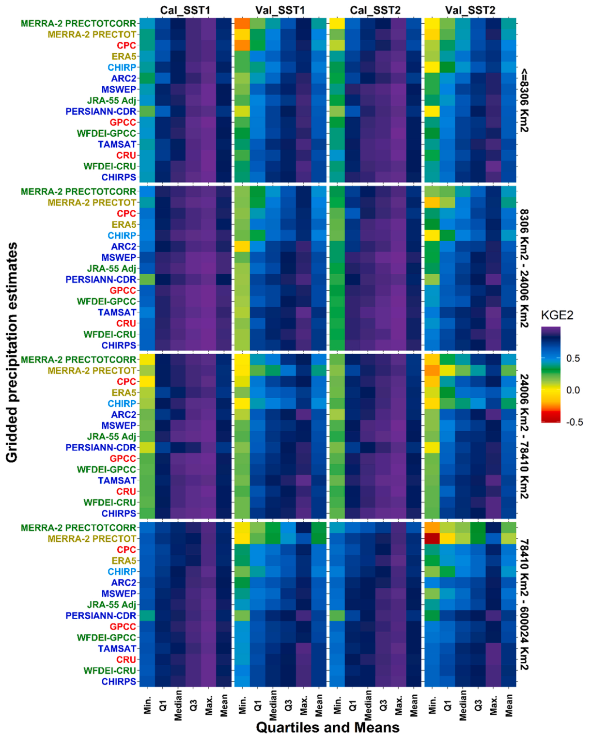
Fig. 8. min/max, quartiles, and means values of KGE2 according to the size of the catchment areas (divided according to surface area quartiles, same number of basins per category) and for different SST's. GPEs are ordered according to the ranking in Table 5, from bottom to the top.
