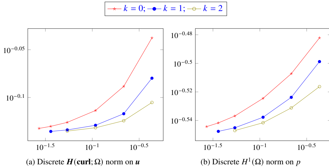
Figure 4: Pressure–flux test of Section 6.2, discrete norms w.r.t. h
