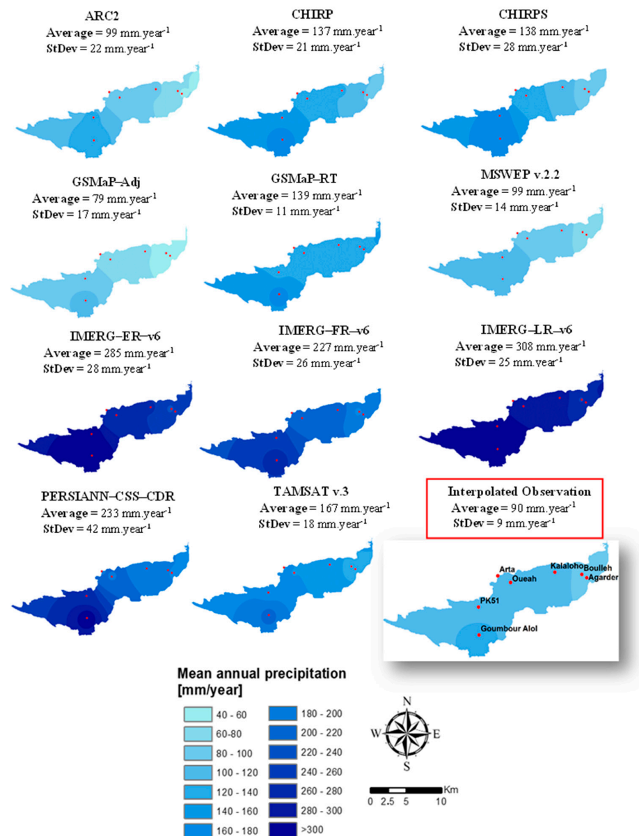
Figure 4. The performance of P datasets in terms of mean annual precipitation compared to the average annual precipitation of the rain gauge stations from 2008–2013.
