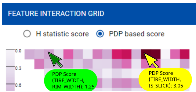
Figure 4. First four rows of the Interaction matrix. The yellow cursor points to the strongest interaction. The name of the features and the interaction score are displayed.
