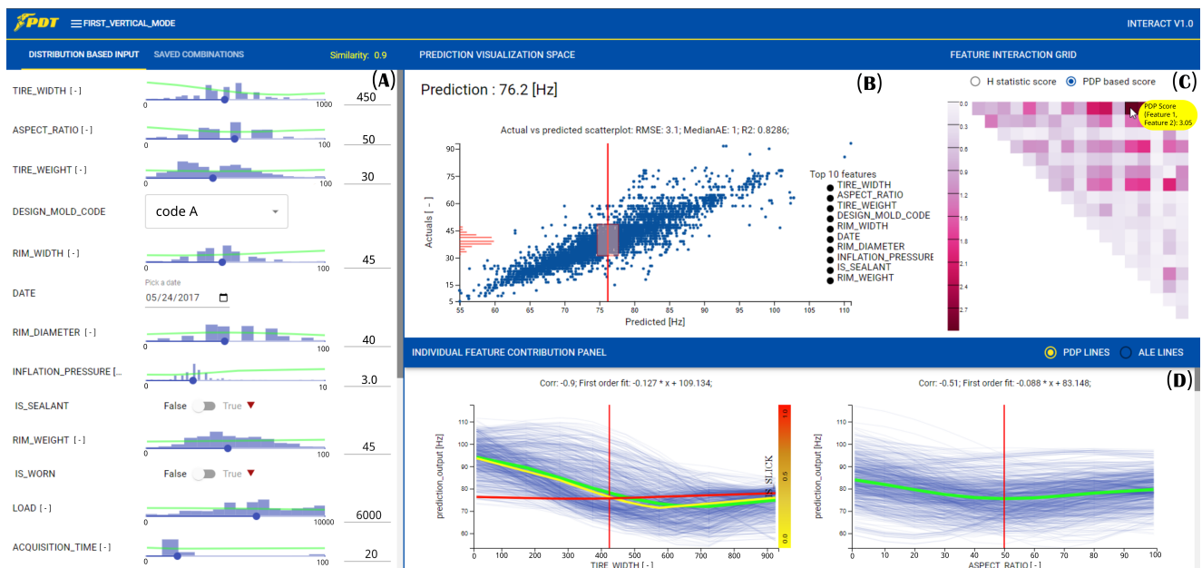
Figure 1. The graphical user interface of INTERACT showing the visualization for the first vertical resonance mode frequency 9 model. A) Data input panel: A set of scented widgets 10 for user control and display of the values of the most important model features. B) Actual vs. predicted plot: a scatterplot augmented with a confidence (red) box and an histogram of the actuals (plotted on the y-axis) for a given prediction. The legend shows the most important model features. C) Feature interaction matrix: Second degree feature interactions based on either the H-statistic or the Partial Dependence (PD) score. D) Individual Conditional Expectation (ICE) plots: a set of linecharts showing the individual contribution of each feature. The yellow to red curves show the interaction between the selected pair of features from (C).
