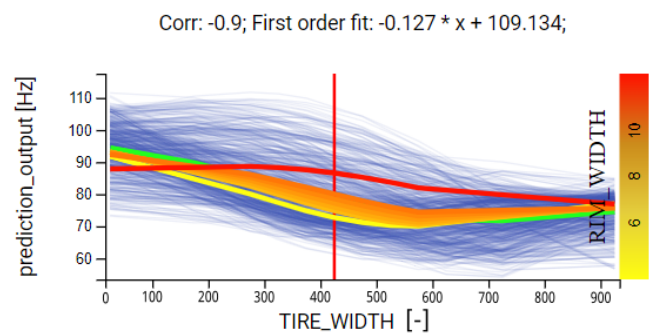
Figure 5. Individual feature contribution panel. ICE lines in blue. PDP in green. A click by the green cursor in Figure 4 populates the plot with second order interaction visualizations - yellow/red lines.
