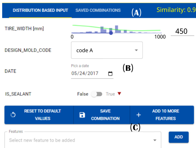
Figure 2. Control pane. A: Two tabs to show either the inputs panel or the comparative analysis panel. The similarity score of the current set of inputs compared to training data is shown in the top-right corner. B: Scented widgets 10 for various data types, sliders, dropdown menus, calendar widgets and toggles. C: Widgets to reset, save combination for comparative analysis or add features.
