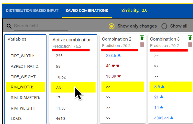
Figure 6. Three combinations showing the same prediction level (above red line) but with different solutions. The reference is the active combination (first column); the scents (triangles) and equality (>>) are with respect to the active combination.
