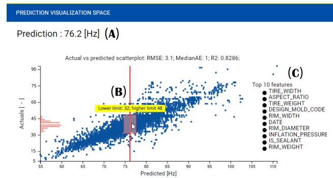
Figure 3. Prediction panel matching Figure 2. A: Prediction for current slider combination. B: Actual vs. predicted plot with linked cursor to current prediction. C: Top 10 most important features of the model.
