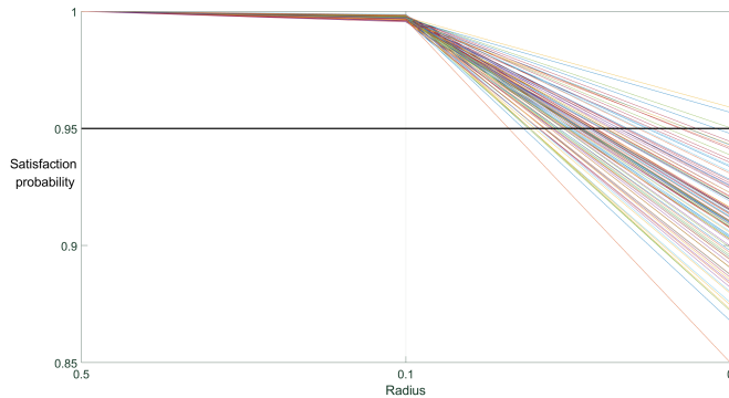
Figure 1: Values of Satisfaction probability \mathbb{P}_{\mathcal{K}_1} under 100 randomly generated Gaussian distributions
