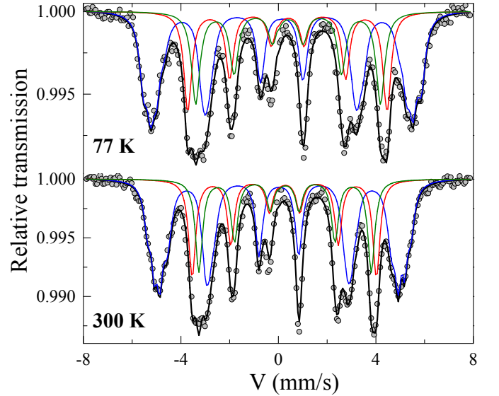
FIG. 8. ^{57}\text{Fe} Mössbauer spectra of \text{Fe}_2\text{RuGe} taken at 300 K (lower panel) and at 77 K (upper panel), respectively.
