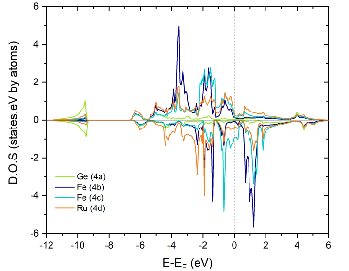
FIG. 10. Projected spin-polarized DOS on each site for the XA-ordered structure.
