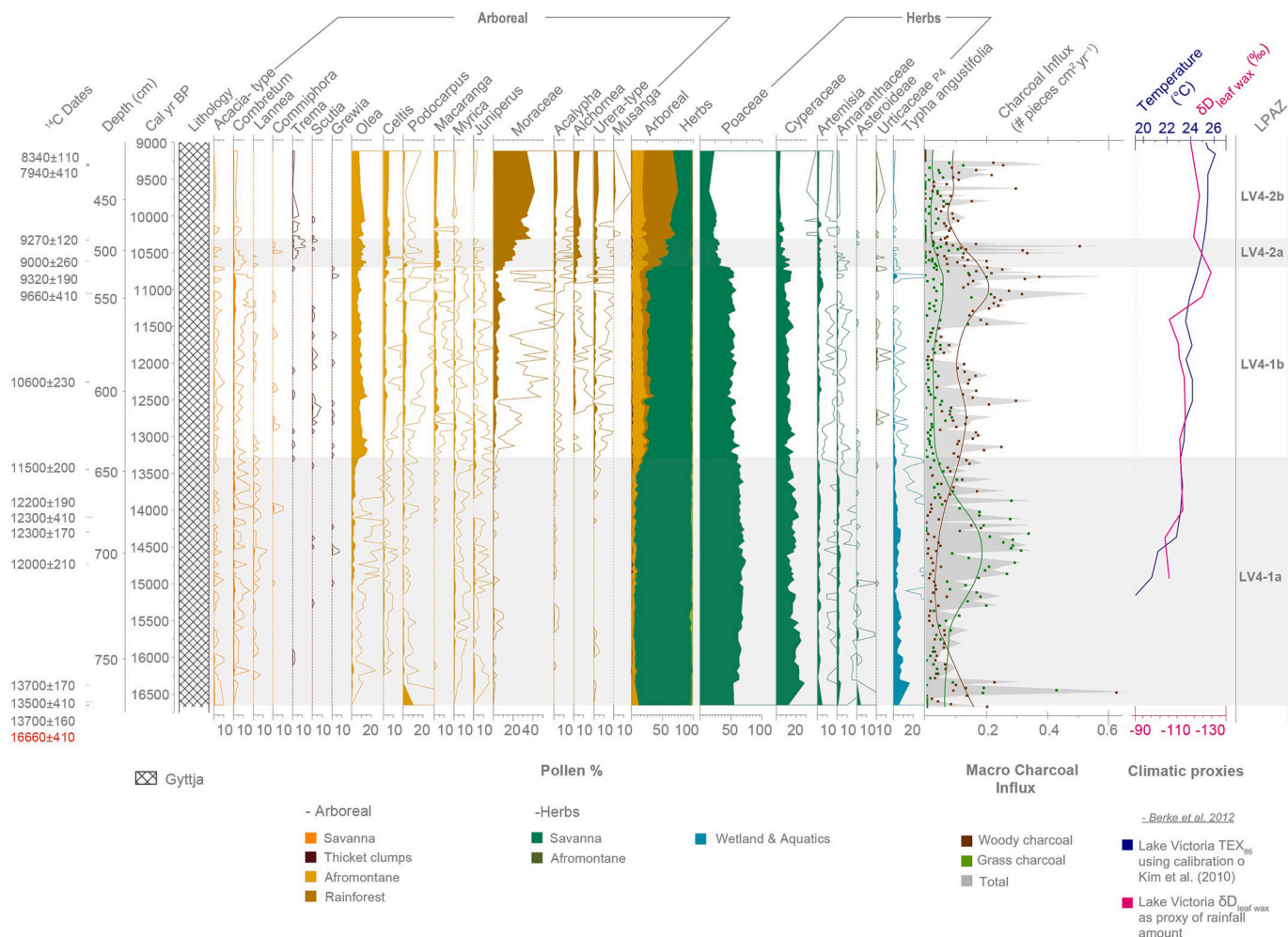
Fig. 3. Selected pollen taxa from Lake Victoria core LV4, charcoal influx, temperature, \delta D_{leaf\ wax} . For the pollen record, the woody taxa are plotted on the left side of the summary curve, in diverse orange-brown shades representing a different ecosystem: Savanna (orange), thicket clumps (brown), Afromontane (dark gold) and tropical rainforest (dark goldenrod). Herb taxa on the right side of the summary curve are plotted in diverse green shades representing a different ecosystem: Savanna (sea green) and Afromontane (olive green). Wetland and aquatics are represented in blue. LPAZ = Local pollen assemblage zones. Empty curves represent a 10× exaggeration. For the charcoal record, the points represent the herb charcoal influx (lime green) and the woody charcoal influx (brown). Continuous lines superimposed on the charcoal data indicate LOWESS smoothing used only for visualization purposes. The gray curve represents the total charcoal influx. Temperature record of Lake Victoria is plotted in °C inferred from TEX 86 using the calibration of Kim et al. (2010), obtained from Berke et al. (2012). \delta D_{leaf\ wax} record from Lake Victoria in ‰, used as proxy of rainfall amount (Berke et al., 2012), more negative values indicate more rainfall. (For interpretation of the references to colour in this figure legend, the reader is referred to the web version of this article.)
