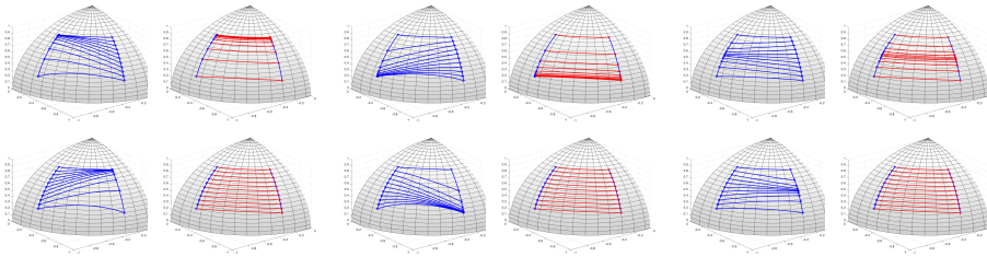
Figure 4: Initial and horizontal geodesics between spherical parameterized curves.
