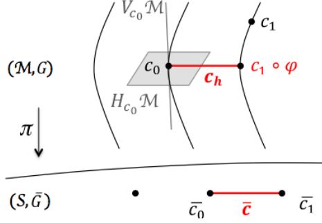
Figure 1: Schematic representation of the shape bundle.
