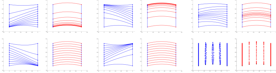
Figure 2: Geodesics between parameterized curves (blue) and corresponding horizontal geodesics (red) in the hyperbolic half-plane, and their superpositions.
