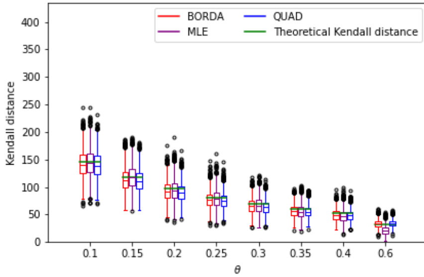
Figure 6: Boxplot of the Kendall distance between \hat{\pi} and \sigma for n = 30 , in the set of parameters P_8 .
