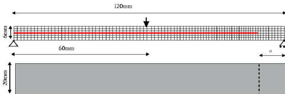
Figure 7 ENF test
