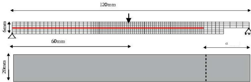
Figure 10 MMF test
