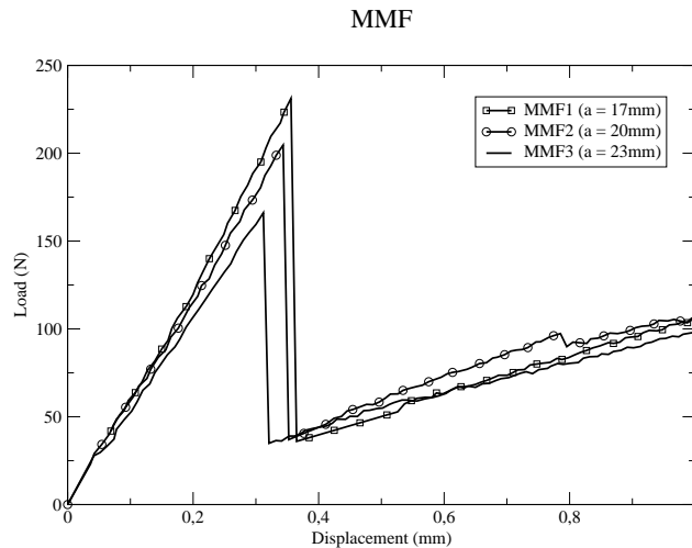
Figure 6 MMF results
