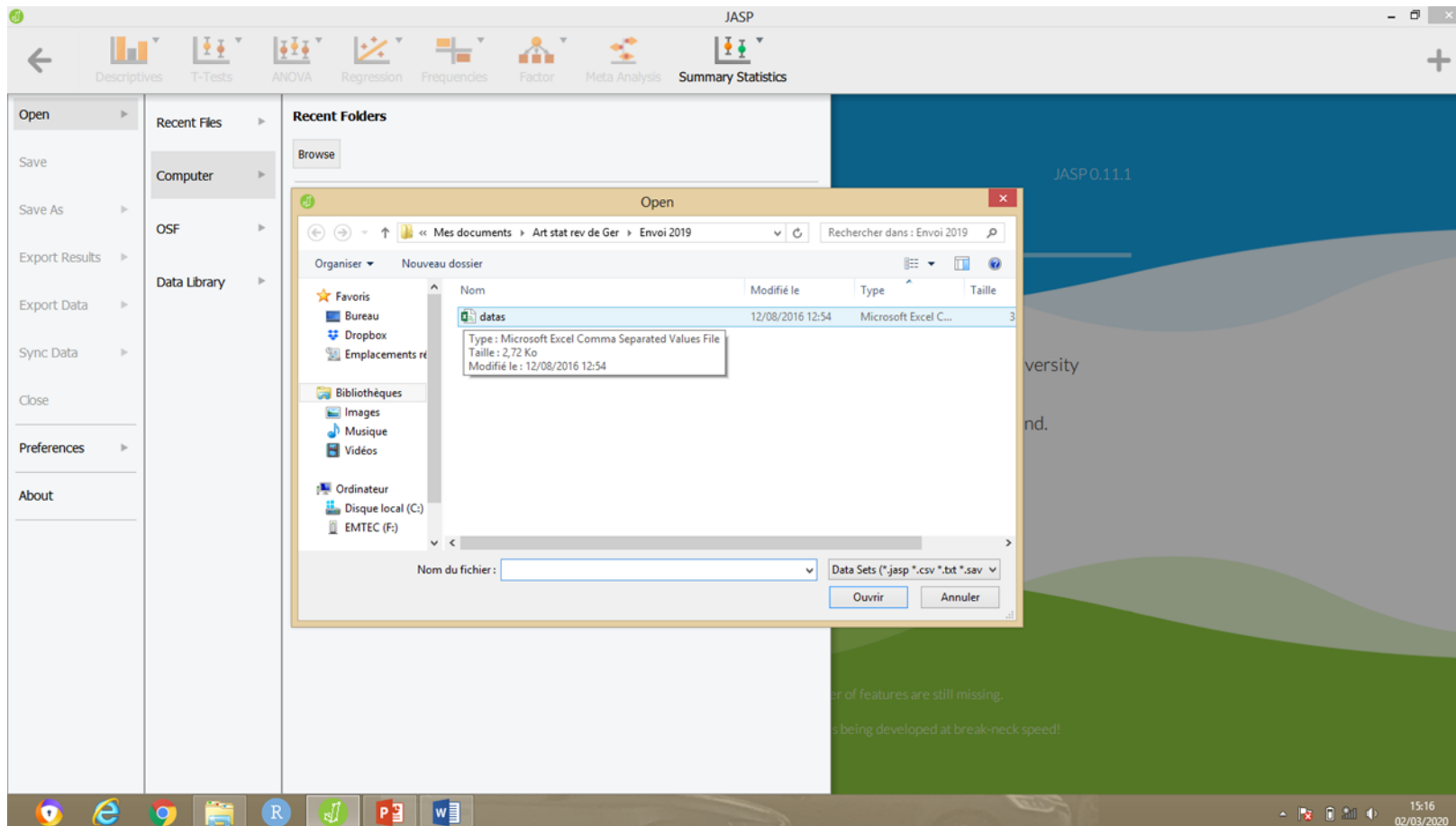
Figure 2 : Importing datas with Jasp
