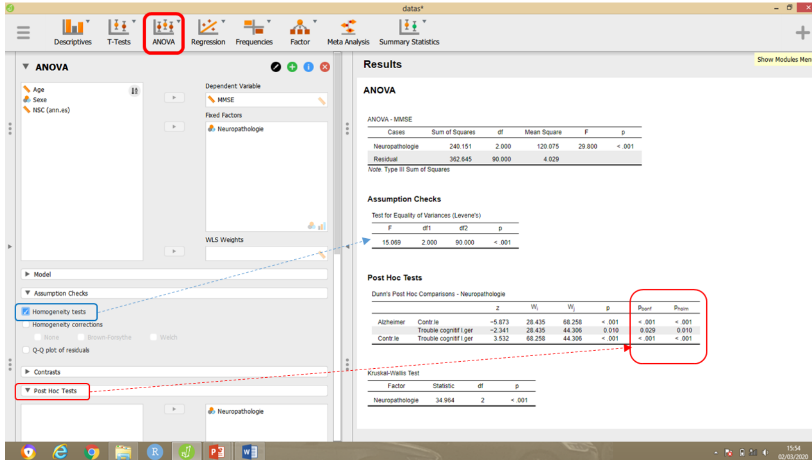
Figure 8 : ANOVA with Jasp
