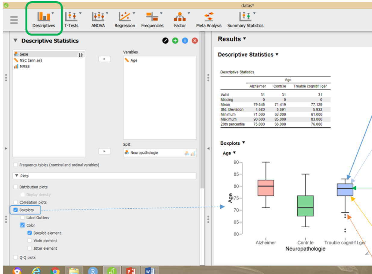
Figure 6 : Descriptive statistics with Jasp (Box plots)
