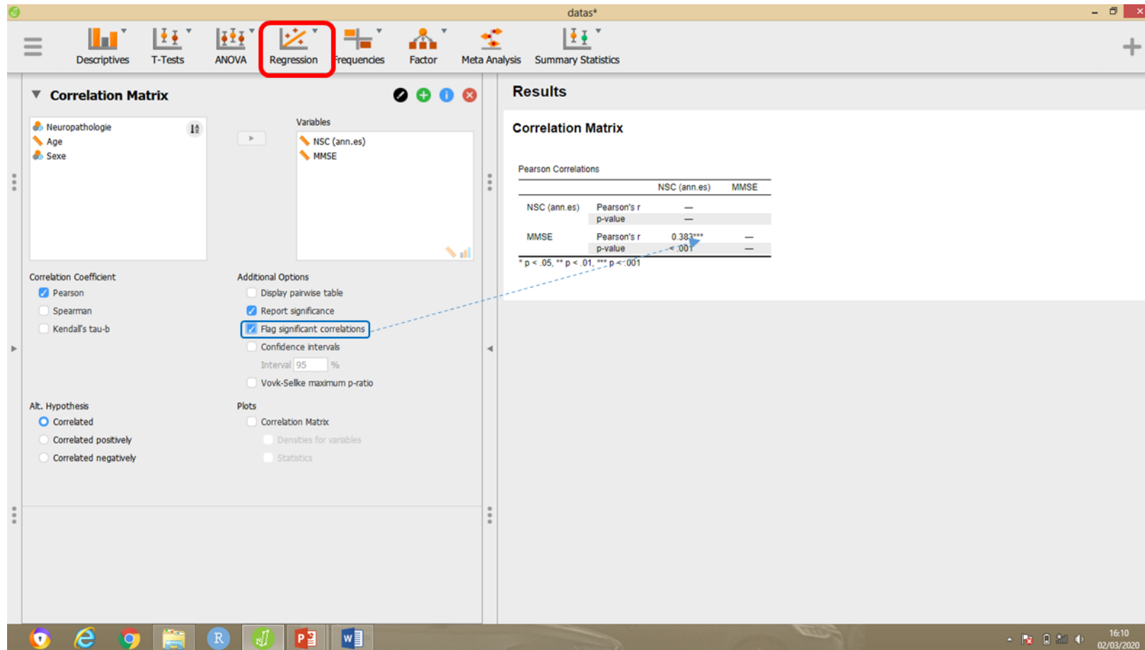
Figure 12 : Correlation with Jasp
