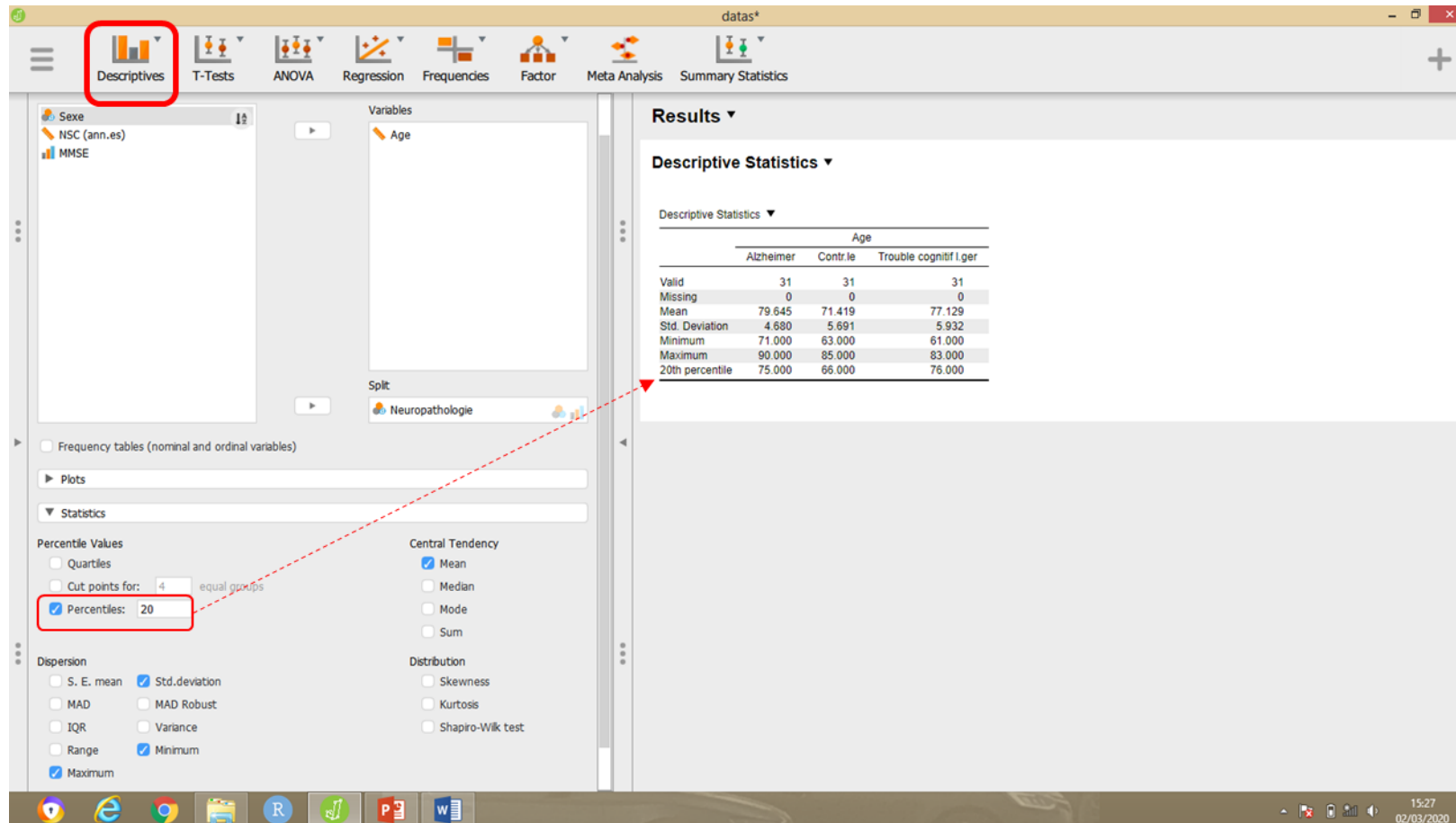
Figure 5 : Descriptive statistics with Jasp
