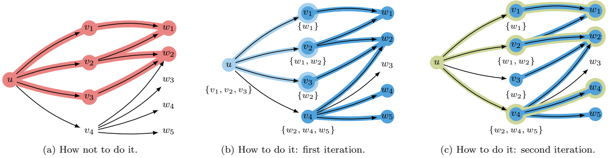
Figure 4: Computing 2-hop neighbours up to threshold 3.
