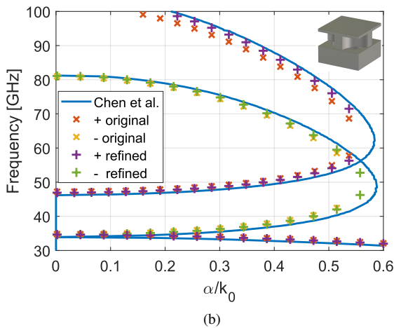
Fig. 14. (a): attenuation in the \overline{\Gamma\overline{X}} region for the glide-symmetric unit cell depicted in the inset. The solutions from 46-59 GHz are located at \Gamma and from 59-87 GHz are a complex mode with the real part presented in Fig. 13. (b): attenuation in the \overline{M\Gamma} region for the mirror-symmetric unit cell depicted in the inset. The solutions from 49-60 GHz were found at M and from 75-100 GHz at \Gamma .
