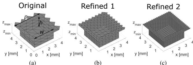
Fig. 8. Meshes of the rectangular holey structure. From left to right they are (a) original, (b) refined 1 and (c) refined 2 meshes. Here, z_{\min} = -1.25 mm and z_{\max} = -0.25 mm. The parameters periodicity are p = 4 mm, depth of hole h = 1.5 mm, the width of hole is w = 3 mm, and the gap is 0.5 mm.
