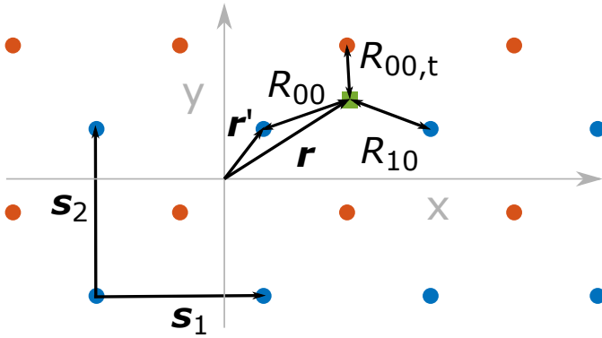
Fig. 1. Higher-symmetric periodic Green's function, represented as double array of point sources. Here, b_1 = b_2 = 0.5 .
