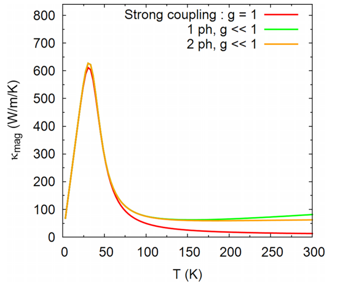
FIG. 5. Thermal conductivity \kappa_{\text{mag}} calculated from Eq. (A1). Different models for the mean-free path are envisaged. For the Umklapp-like mean-free path, we use g = 1 , \omega^* = 204 K. For the weak-coupling limit, we use g = 0.025 , \omega^* = 300 K. In all calculations, n_d = 35 \times 10^{-7} and J = 2600 K.
