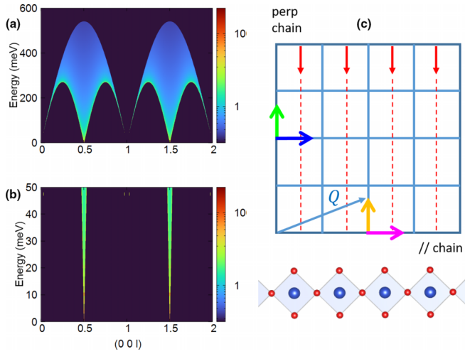
FIG. 1. Panels (a) and (b) display the calculated two-spinon continuum in different energy ranges, using the full scale in panel (a) up to 600 meV, because of the high value of J_{AF} ( =2600 K in the calculation shown), and up to 50 meV in panel (b) to compare with the typical energies of phonon modes. Panel (c) shows a sketch of the reciprocal space probed in the present neutron-scattering experiments. The plane is spanned by the direction of the spin chains ( c axis in \text{SrCuO}_2 , b axis in \text{Sr}_2\text{CuO}_3 and \text{Ca}_2\text{CuO}_3 ) and a perpendicular direction ( a axis in \text{SrCuO}_2 , c axis in \text{Sr}_2\text{CuO}_3 and \text{Ca}_2\text{CuO}_3 ). The red arrows which terminate as dotted lines indicate the zone boundaries where the two-spinon continuum goes soft. Orange (green) arrows show the scan directions allowing to probe transverse (longitudinal) phonon modes propagating perpendicular to the chains. Blue (magenta) arrows show the directions to probe transverse (longitudinal) phonon modes propagating along the chains.
