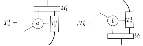
Figure 8. One full iteration for the edge tensors T_a^1 and T_b^1 , Eqs. (9, 10, 12, 13). The other edge tensors are updated similarly.
