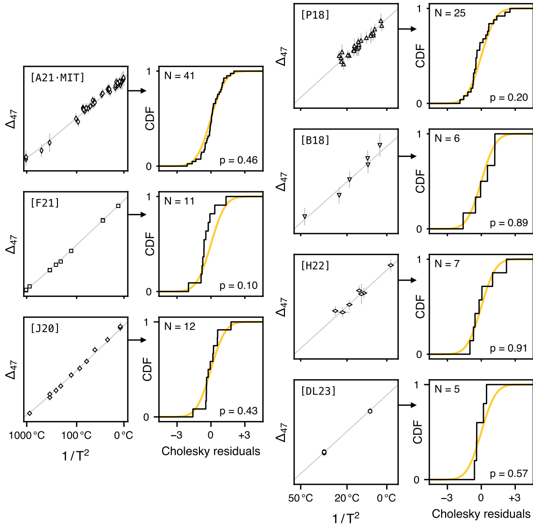
Figure 15 — Kolmogorov-Smirnov tests of normality for the Cholesky residuals of each individual calibration relative to the combined regression [0GLS23]. Left-hand plots show the data points, with 95 % error bars, for each data set, along with the combined regression line. Right-hand plots show the cumulative distribution of Cholesky residuals, with the number of observations and p-value for a Kolmogorov-Smirnov test of normality with mean of zero and variance of one. All data sets have a distribution of Cholesky residuals which is statistically indistinguishable from the expected Gaussian distribution (section 4.3.2). See Appendix A for reprocessing details.
