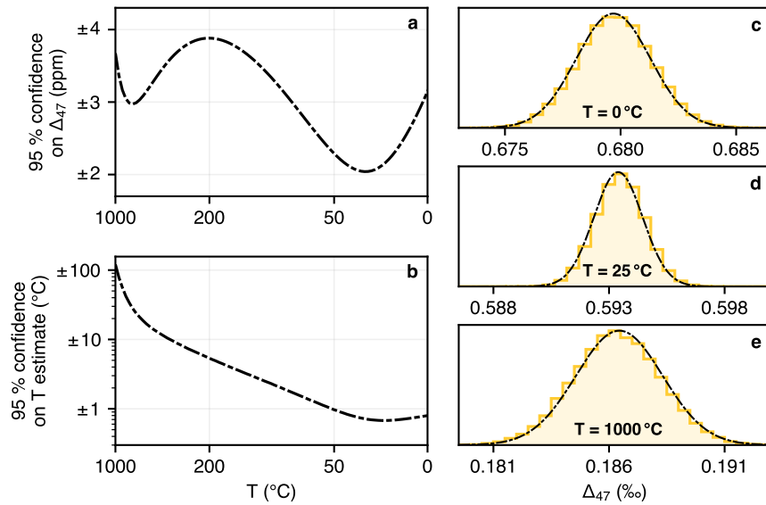
Figure 17 — Regression confidence limits on the [0GLS23] calibration. Left panels: confidence limits on \Delta_{47} and T estimates as a function of T (x axis is scaled as 1/T^2 ). Right panels: Quasi-Monte Carlo simulations of \Delta_{47} uncertainties at three different values of T , confirming the applicability of our first-order propagation methods. See Appendix B.2 for computation details.
