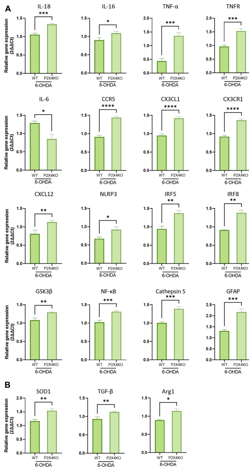
FIGURE 6 Detection of pro- (A) and anti-inflammatory (B) markers in the PI of 6-OHDA-WT and 6-OHDA P2X4KO mice. All data are expressed as relative gene expression, mean ± SEM (n = 3–8 mice per group), and were analysed with a two-tailed Unpaired t -test (* p < 0.05; ** p < 0.01; *** p < 0.001; **** p < 0.0001).
