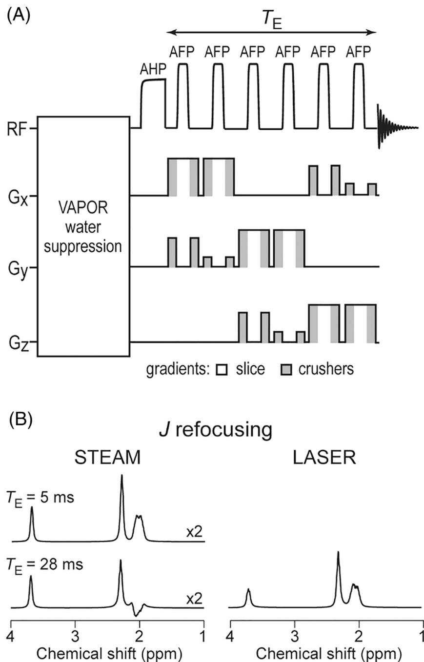
FIGURE 2. LASER sequence. A, LASER sequence with RF and gradient pulses shown schematically. Volume selection with LASER is performed with AFP pulses. Pulsed field gradients are used for suppressing outer-volume signals (gray shading) and for slice selection (white). B, Simulated scalar coupling evolution of glutamate at 9.4 T for STEAM sequence at T_E = 5 ms and 28 ms, and LASER sequence at T_E = 28 ms. The successive application of multiple AFP pulses in the LASER sequence suppresses J evolution in coupled spin systems. The vertical scale for the STEAM sequence has been multiplied by 2
