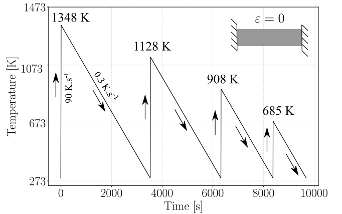
Fig. 14. Thermomechanical loading path for the Satoh test.
