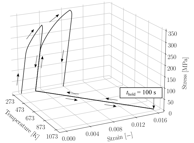
(a) Stress vs. strain vs. temperature.
