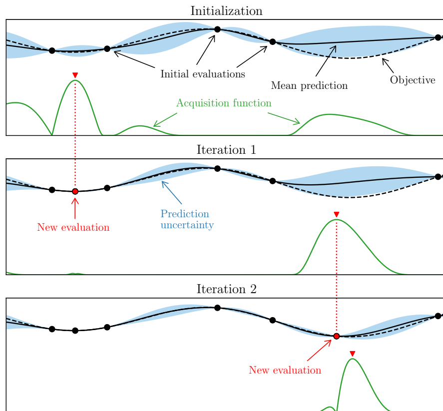
Figure 8: Illustration of the Bayesian optimization for the minimization of a simple 1D function.
