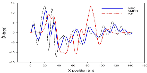
Fig. 11: Heading rate for S_{c2} .
