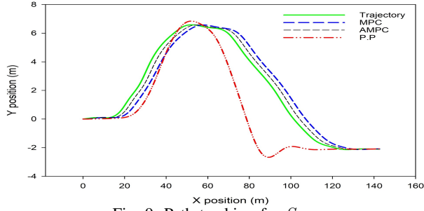
Fig. 9: Path tracking for S_{c2} .
