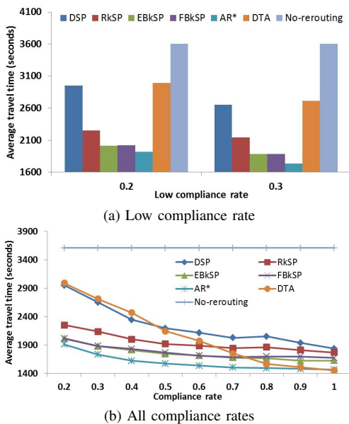
Fig. 14: Average travel time as a function of the compliance rate on Brooklyn network. ( L=3 , k=4 , urgency= ACI , period= 450s , \delta=0.7 , \beta=0.05 )
