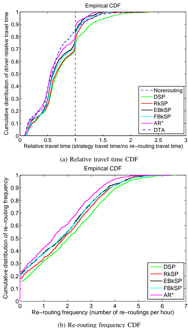
Fig. 10: CDF of relative travel time and re-routing frequency per hour on Brooklyn network. ( L=3 , k=4 , urgency= ACI , period=450s, \delta=0.7 , \beta=0.05 )
