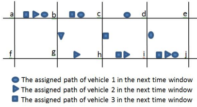
Fig. 2: AR^* re-routing example. All road segments have same weight and \beta = 0.5 .
