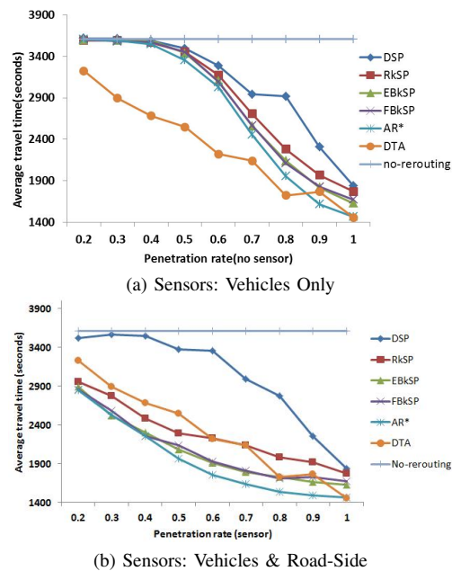
Fig. 15: Average travel time as a function of the penetration rate on Brooklyn network ( L=3 , k=4 , urgency= ACI , period= 450s , \delta=0.7 , \beta=0.05 )
