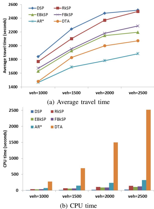
Fig. 12: The average travel time and CPU time for Brooklyn network for different traffic densities ( L=3 , k=4 , urgency= ACI , period=450s, \delta=0.7 , \beta=0.05 )
