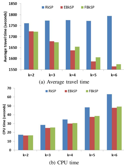
Fig. 13: Average travel time, CPU time for RkSP, EBkSP and FBkSP as function of k for the Brooklyn network ( L=3 , k=(2, 3, 4, 5, 6) , urgency= ACI , period=450s, \delta=0.7 )
