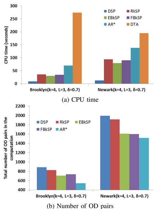
Fig. 11: CPU time and number of origin-destination pairs for both networks ( L=3 , k=4 , urgency= ACI , period=450s, \delta=0.7 , \beta=0.05 )
