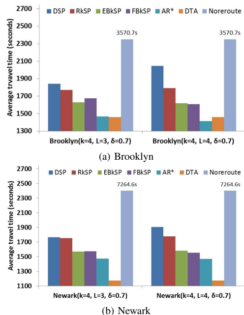
Fig. 7: Average travel time ( L=(3,4) , k=4 , urgency= ACI , period=450s, \delta=0.7 , \beta=0.05 )
