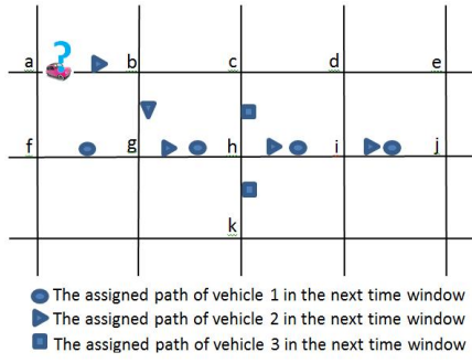
Fig. 3: A EBkSP re-routing example. All segments have same weight.
