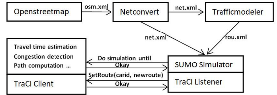
Fig. 5: The simulation process
