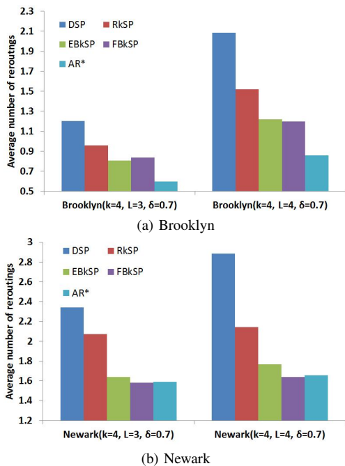
Fig. 8: Average number of re-routings ( L=(3,4) , k=4 , urgency= ACI , period=450s, \delta=0.7 , \beta=0.05 )
