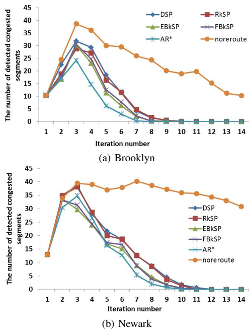
Fig. 9: Number of congested road segments as function of the number of iterations. ( L=3 , k=4 , urgency= ACI , period=450s, \delta=0.7 , \beta=0.05 )
