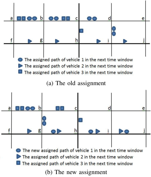
Fig. 4: A FBkSP example. \omega_{fg} = \omega_{gh} = \omega_{hi} = \omega_{ij} = \omega_{ch} = 1 , \omega_{ab} = \omega_{bc} = \omega_{cd} = \omega_{de} = \omega_{af} = \omega_{bg} = \omega_{di} = \omega_{ej} = 2 .
