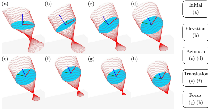
Fig. 7. Simulations of the process of lens reorientation and focus, with polar angle \varphi_0 = 5/6\pi and azimuthal angle \theta_0 = 1/6\pi
