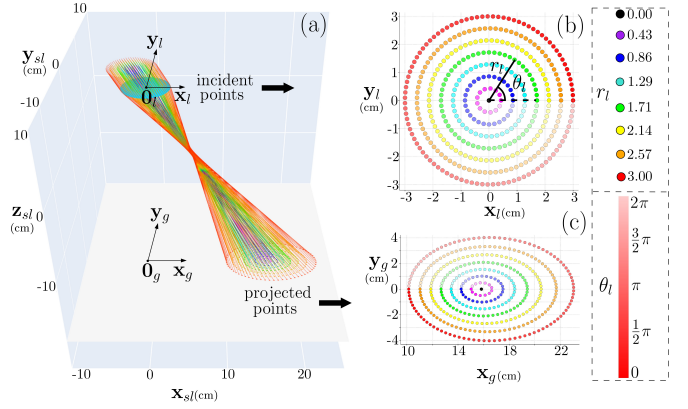
Fig. 5. Illustration of the geometrical characteristics of the projected points. Remember to change r_l to r_{l_i}
