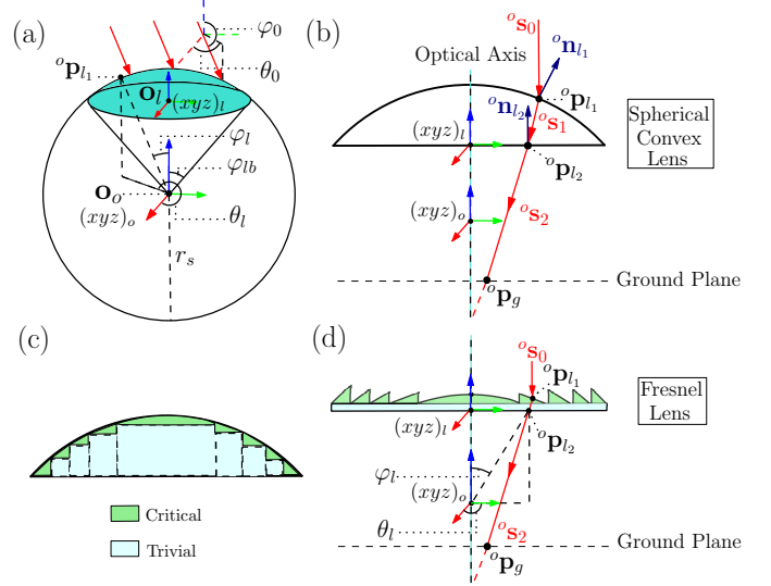
Fig. 4. Ray tracing and structure diagrams of the plano-convex lens and the Fresnel lens.
