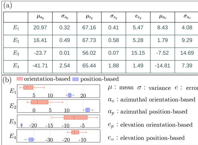
Fig. 12. A quantitative evaluation of the performance of different estimation methods. The position-based method outperforms the orientation-based method, in terms of accuracy and stability.
