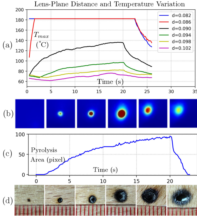
Fig. 8. Experiments designed to determine the parameters for the motion control algorithm. (a) Solar concentration experiments with fixed duration and varying lens-plane distance. (b) Representative thermal images captured before, during and after the wood pyrolysis process; (c) Variation of the pyrolysis region with respect to time; (d) The size of a carbonized point can be controlled by the selection of \bar{N}_p .
