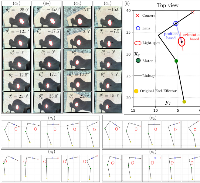
Fig. 11. Experiments evaluating the performance of the solar orientation estimation utilizing different geometric features. (a 1 )-(a 4 ) include images captured from four experiments with varying lens yaw angles, and (c 1 ) - (c 4 ) show the corresponding robot configuration from the top view. (b) annotates the components in the robot configuration visualization.
