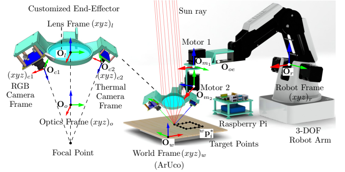
Fig. 3. A schematic of the system with relevant frames. The system is composed of a 3-DOF robot arm with two additional motors (controlled by a Raspberry Pi ), manipulating a customized end-effector. The end-effector carries a spherical Fresnel lens, an RGB camera, and a thermal camera. An ArUco marker defines the World Frame.
