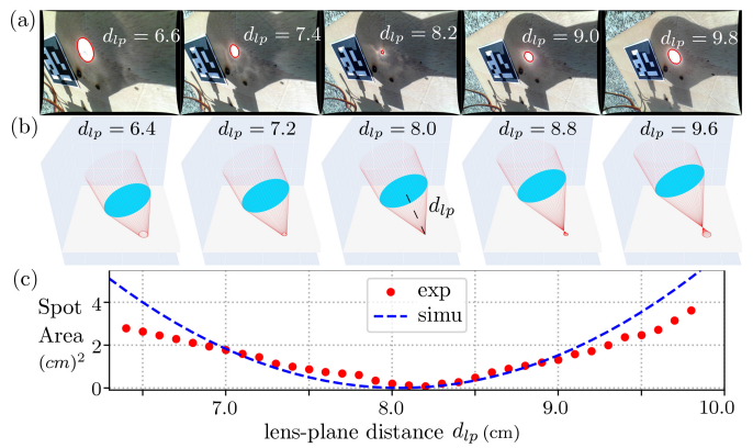
Fig. 10. Image-based focal length calibration experiment. (a) includes snapshots of captured light spot and extracted contour; (b) shows the corresponding lens-plane configuration in the developed simulation; (c) shows the comparison between the light spot area from the real images and the simulation.
