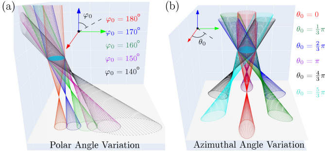
Fig. 6. The effect of the solar orientation variation on the light spot when the lens plane is parallel to the ground plane.
