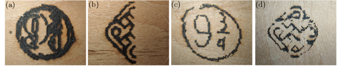
Fig. 15. Examples of failed solar paintings, which are caused by (a) inappropriate feature selection in the path planning stage, (b) the lens being shadowed as the solar orientation changed, (c) inaccurate solar orientation estimation and (d) a cloudy situation when N_p is set too small.
