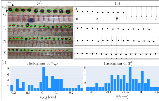
Fig. 13. Validation of the positional accuracy of the developed system. The mean of the horizontal error is 0.099 cm, and the mean of vertical error is 0.061 cm.
