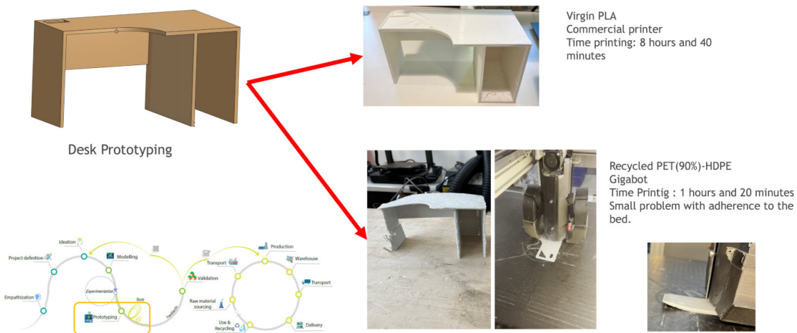
Figure 35: Prototype of the desk
