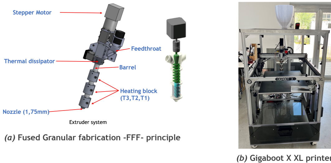
Figure 13: Fused Granular Fabrication fabrication
