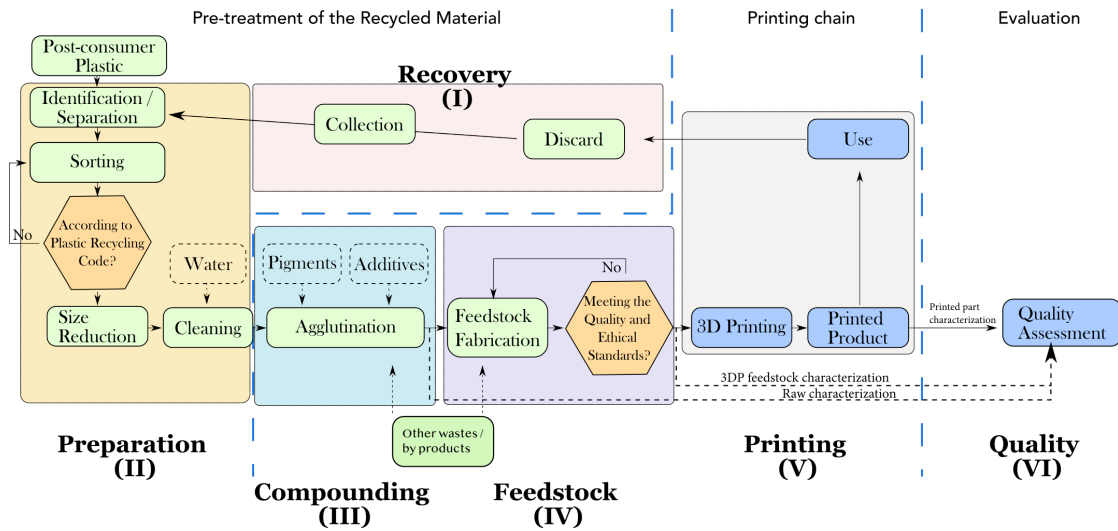
Figure 6: Distributed recycling via additive manufacturing (DRAM) approach (Cruz Sanchez et al., 2020)
