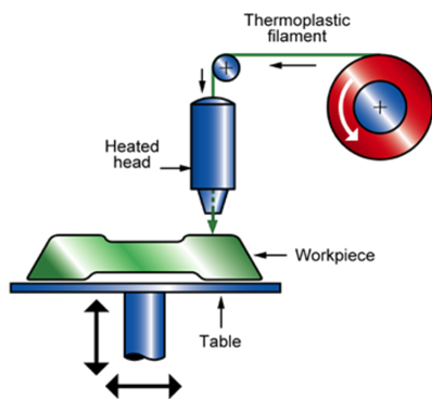
(a) Fused filament fabrication -FFF- principle
