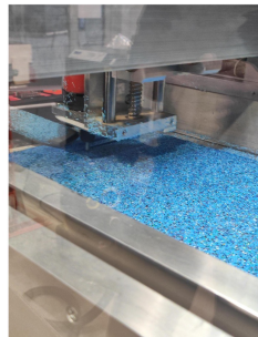
Figure 28: Post-processing activities for the injection molding and 3D printing processes
