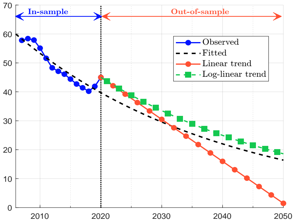
Figure 9.24: Log-linear carbon trend (Example 38)
