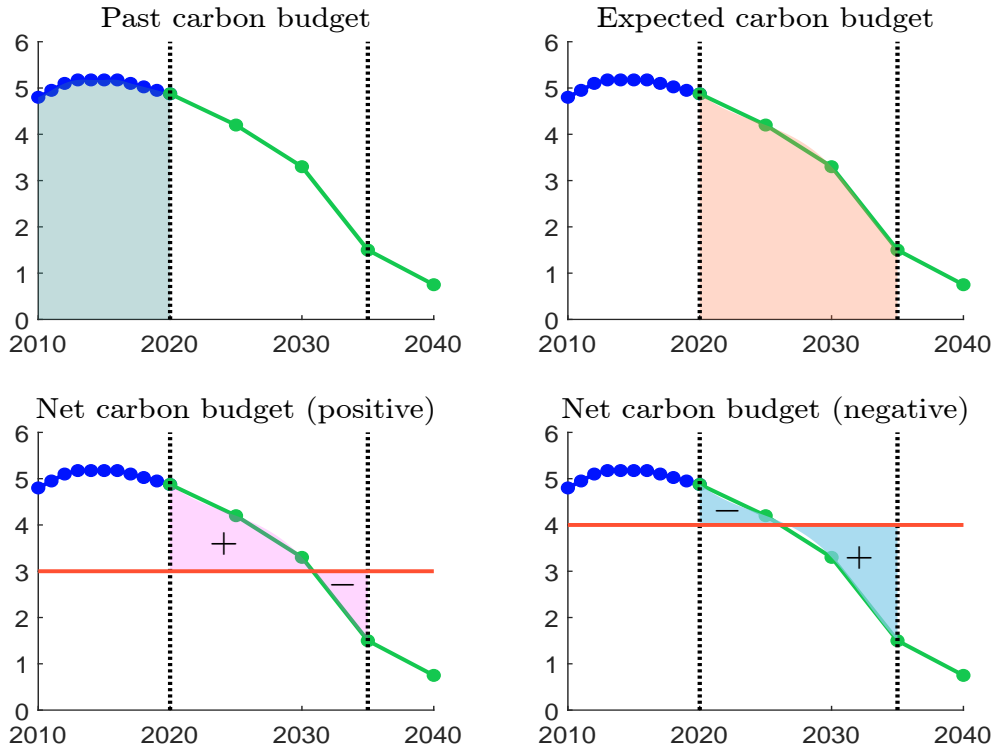
Figure 9.20: Past, expected and net carbon budgets (Example 36)
