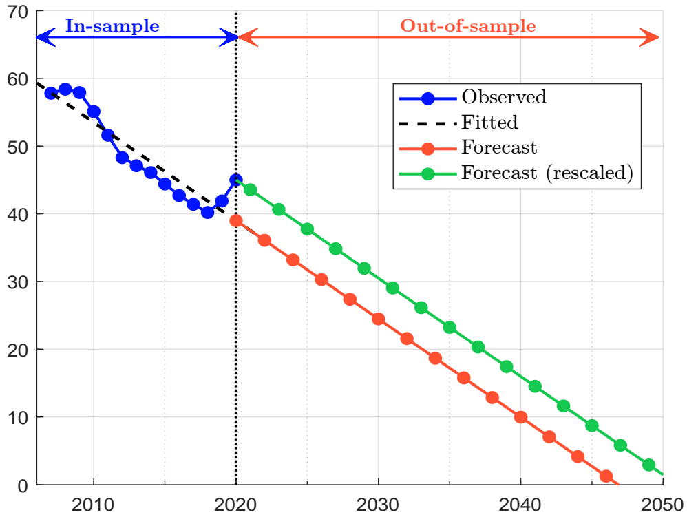
Figure 9.23: Linear carbon trend (Example 38)
