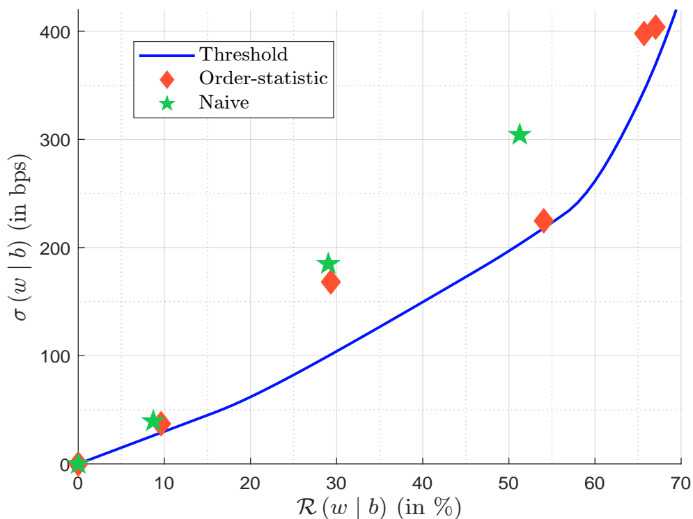
Figure 11.3: Efficient decarbonization frontier (Example 46)
