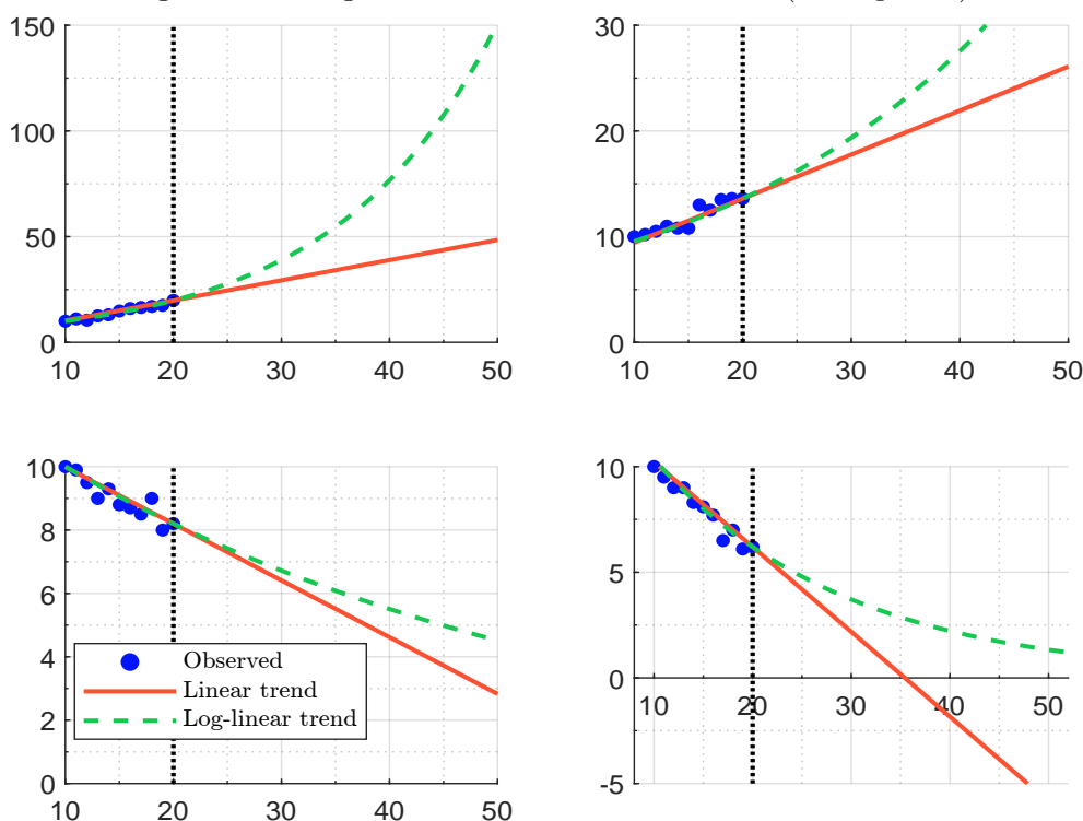
Figure 9.25: Log-linear vs. linear carbon trend (Example 39)
