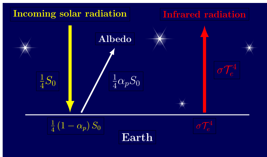
Figure 8.37: Zero-order model
