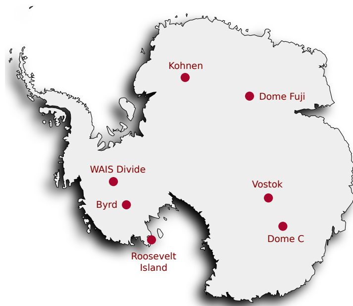
Figure 8.11: Antarctica deep drilling sites
