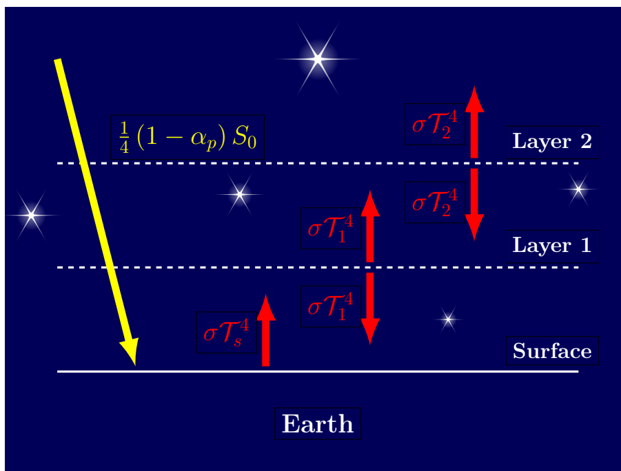
Figure 8.39: Two-layer model
