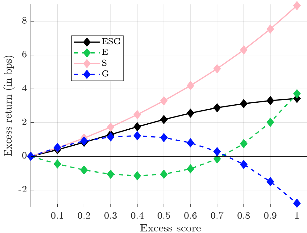
Figure 3.35: Annualized excess return in bps of ESG optimized portfolios (EUR IG, 2014–2016)
