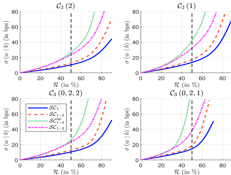
Figure 11.9: Impact of \mathcal{C}_2 and \mathcal{C}_3 constraints (MSCI World, June 2022)
