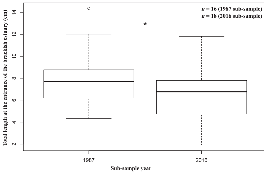
FIGURE 7 Total length of allis shad ( Alosa alosa ) juveniles from the 1987 and 2016 subsamples when entering the brackish estuary of the Gironde-Garonne-Dordogne system. The asterisk indicates a significant difference between subsamples ( p < 0.05 ). The boxes represent medians, first and third quartiles. Values greater than 1.5 times the interquartile range away from the median are represented by an empty circle.
