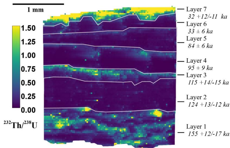
275 Figure 5: definition of the different layers of SOY-02Exo on the ^{232}\text{Th}/^{238}\text{U} ratio mapping obtained by fsLA-single collector-ICP-SFMS. The layer numbers are indicated on the figure, starting from 1 for the layer in contact with the Endo part to 7 for the surface layer. The ages on the right are the STRUTages computed according to Roy-Barman and Pons-Branchu (2016) and provided at 95% CL. 280
