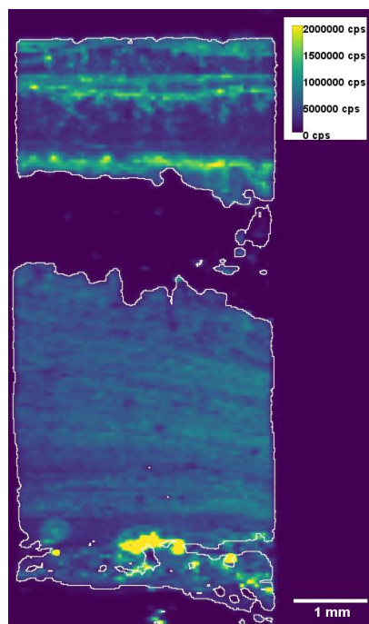
(a) ^{24}\text{Mg}
