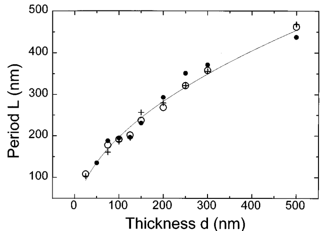
FIG. 6. Period L of the stripe pattern as a function of Co film thickness d (see text). (○) demagnetized parallel, (●) demagnetized perpendicular, (+) magnetized parallel.
