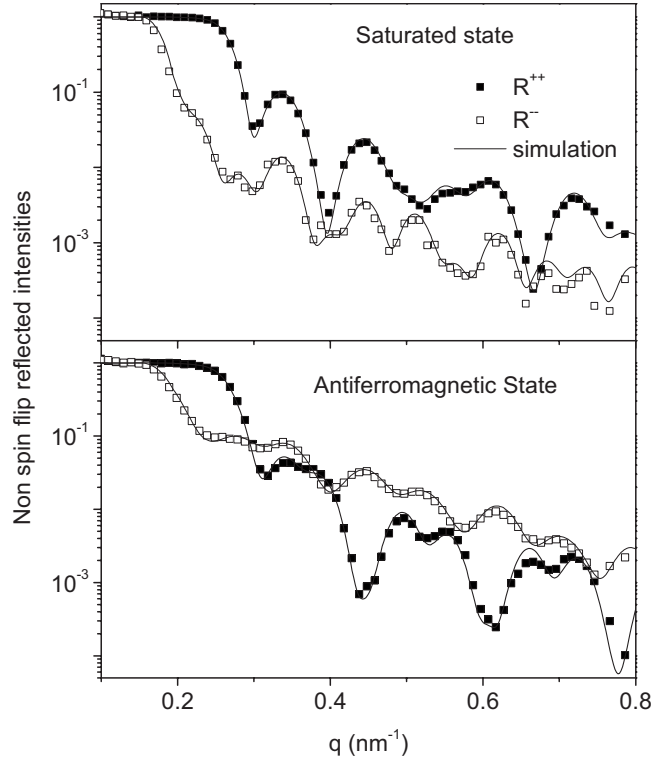
FIG. 5. Non-spin-flip reflectivities R^{++} and R^{--} measured for an applied field of 900 and 90 G along the EA1. These field values correspond to the saturated and the antiferromagnetic states, respectively. The solid lines are simulations.
