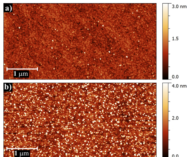
FIG. 3. AFM images of \text{Co:TiO}_2 films grown (a) with and (b) without the \text{TiO}_2 buffer layer.
