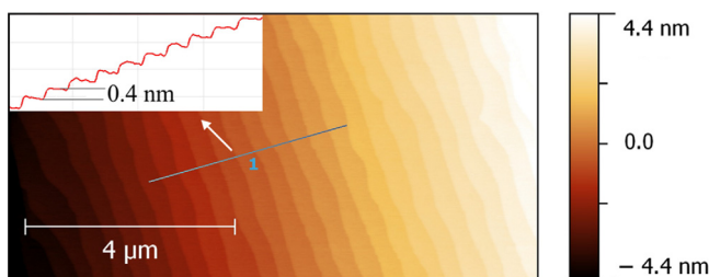
FIG. 1. AFM image of the \text{SrTiO}_3 substrate surface after the chemical treatment and annealing, showing the formation of large, atomic flat, well regulated terraces. The inset shows a height profile corresponding to the indicated line.
