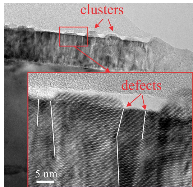
FIG. 6. Cross-sectional bright field image of the Co:TiO 2 unbuffered film. Inset shows a high resolution TEM image of the emphasized region containing surface clusters.
