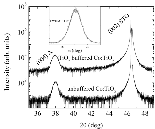
FIG. 2. 2\theta - \omega x-ray diffraction selected area scans of 40 nm thick \text{Co:TiO}_2 films with and without the 5 nm thick \text{TiO}_2 layer. The scans were shifted vertically for better visibility. The inset shows the XRD rocking curve for the buffered film.
